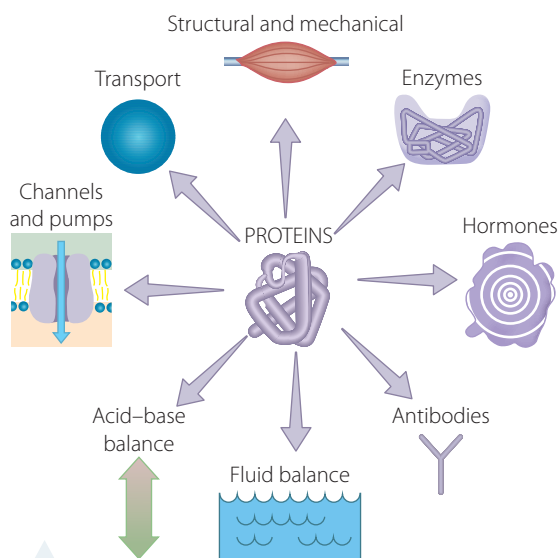
FIGURE 13.18 Protein functions
