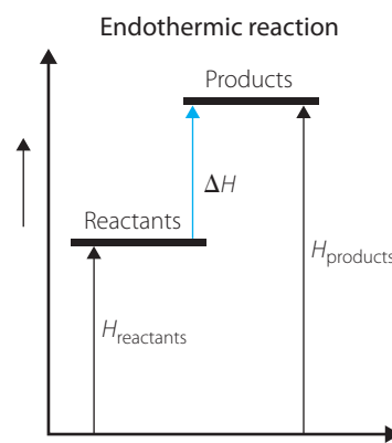
FIGURE 5.7 In an endothermic reaction, energy is absorbed since energy of reactants is less than energy of products.
