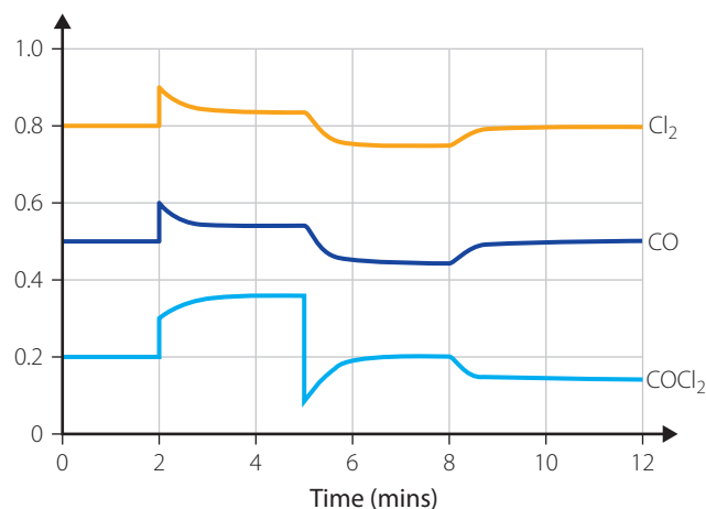
FIGURE 2.22 Closed system of a mixture of gases
