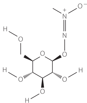
FIGURE 4.13 The toxin, cycasin, methylazoxymethanol glucoside, is commonly found in cycads.
