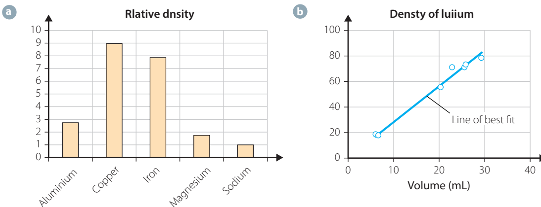
FIGURE 1.12 a A column graph can be used for discrete data; b a scatter graph is used to show a mathematical relationship between continuous data.
