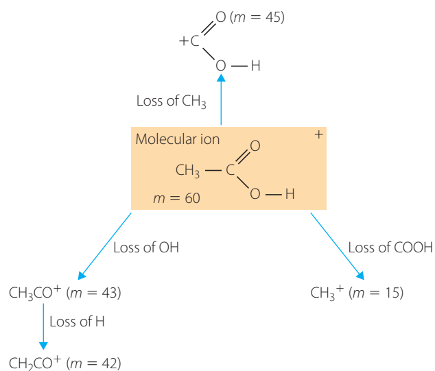
FIGURE 15.7 Simplified fragmentation pattern of molecular ion CH_3COOH^+
