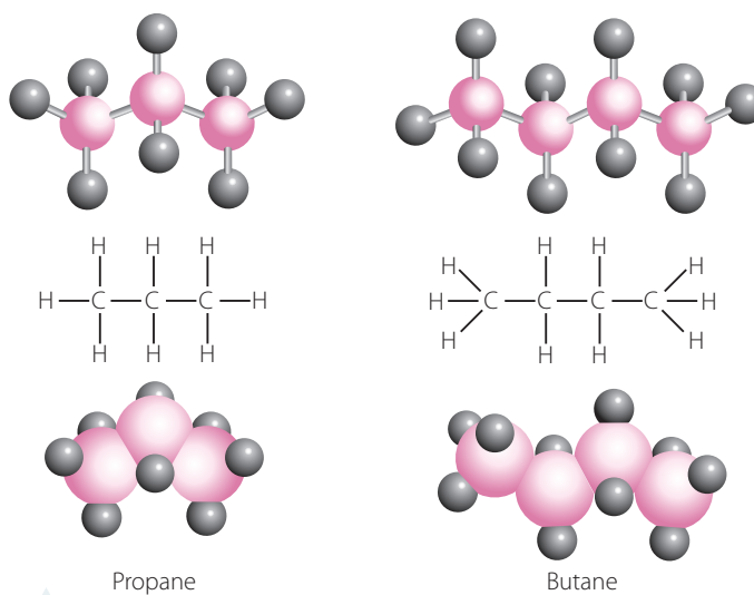
FIGURE 8.6 Models and structural formulae for propane and butane
