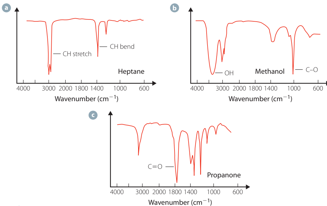
FIGURE 15.26 Infrared spectra of heptane, methanol and propanone ( \text{CH}_3\text{COCH}_3 ). The broad trough at around 3200\text{ cm}^{-1} is characteristic of an alcohol \text{—OH} stretch. The vibrations that cause the major absorption bands are identified.
