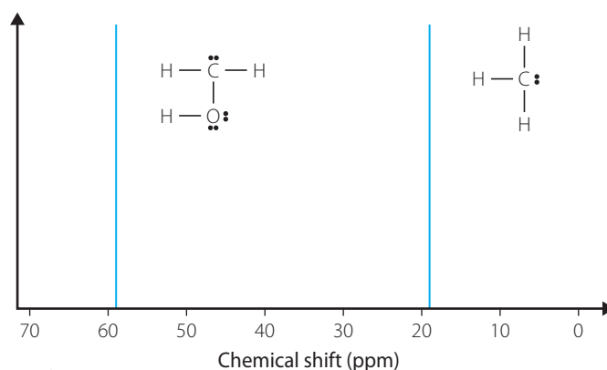
FIGURE 15.23 13 C NMR spectrum of ethanol
