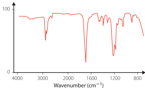
FIGURE 15.34 Infrared spectrum of compound X
