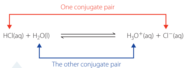
FIGURE 6.4 Conjugate acid–base pairs
