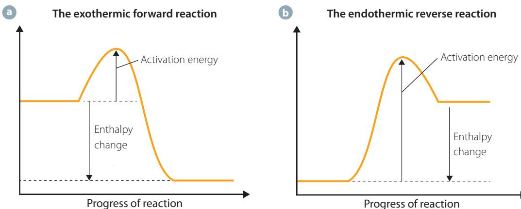
FIGURE 2.20 Comparing the activation energy for the forward and reverse reactions of: reactants \rightleftharpoons products + energy. Note how the activation energy for the exothermic reaction is less than the activation energy for the endothermic reaction.
