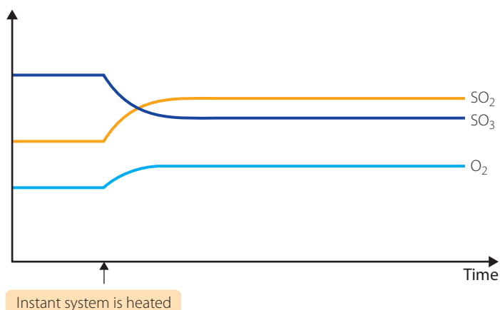
FIGURE 2.19 Concentrations with a change in temperature for the reaction 2\text{SO}_2(\text{g}) + \text{O}_2(\text{g}) \rightleftharpoons 2\text{SO}_3(\text{g})
