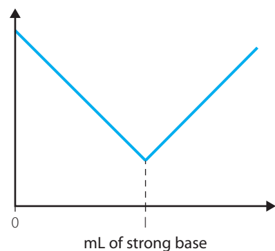
FIGURE 7.11 Conductivity graph for a titration involving a strong acid and a strong base
