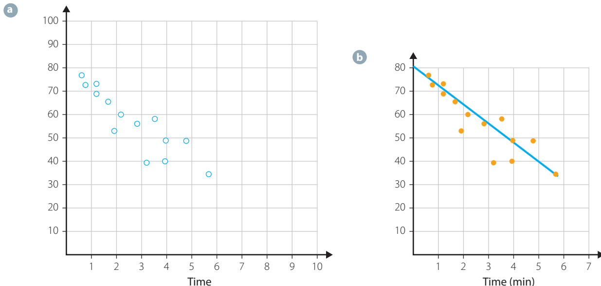
FIGURE 1.8 a A poor example of a graph; b a good example of a graph of the same data. How many differences can you see?
