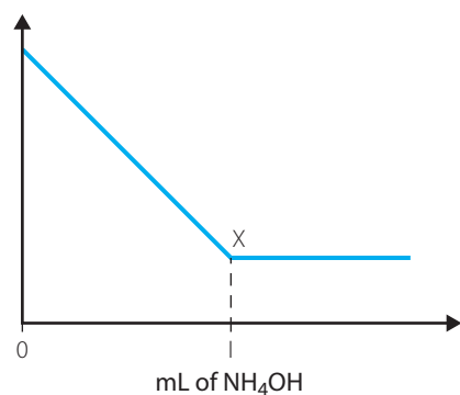
FIGURE 7.22 Conductivity graph for a titration between \text{H}_2\text{SO}_4 and \text{NH}_4\text{OH}
