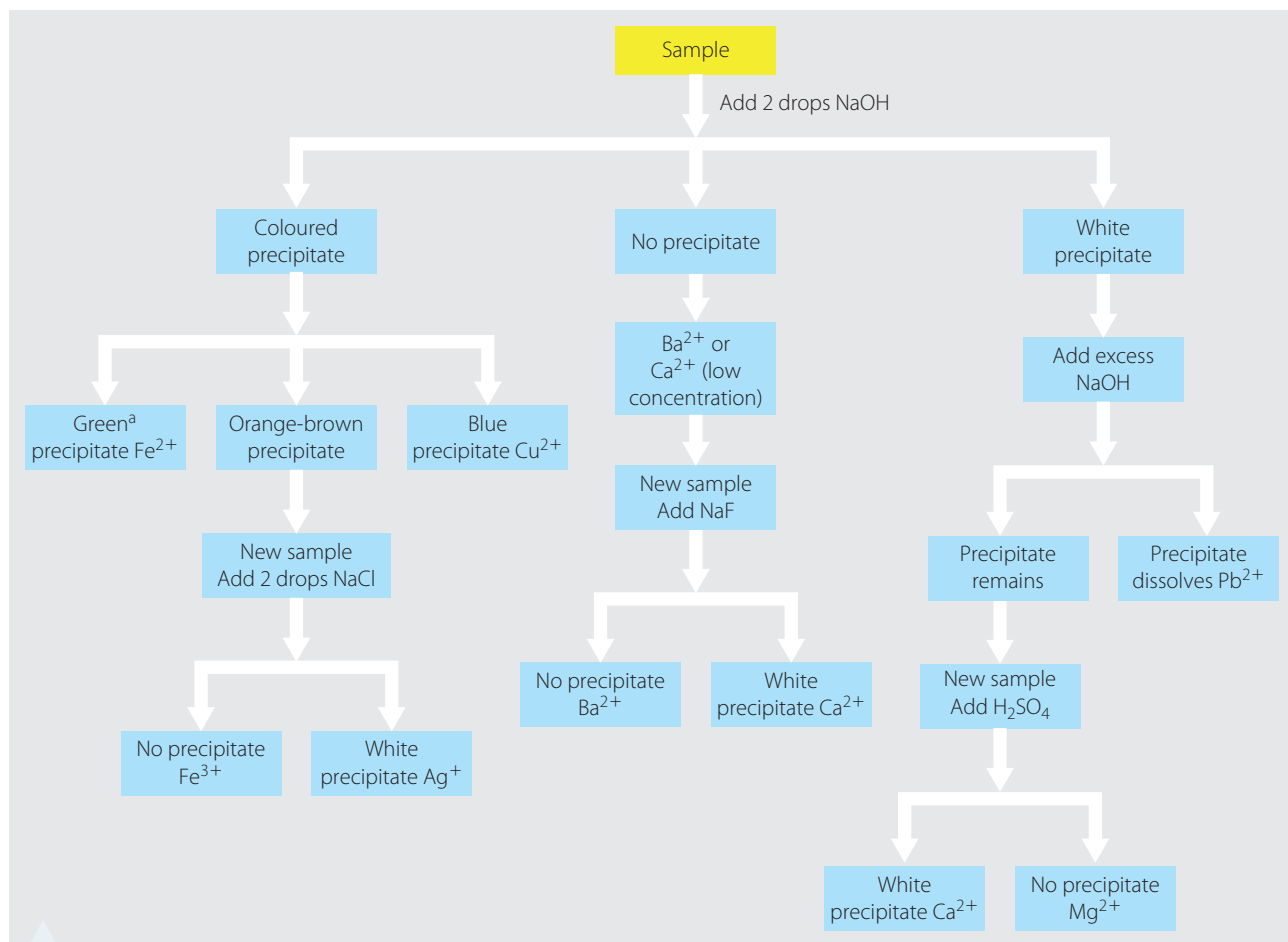
FIGURE 14.6 Flow chart for identifying the cation in a single cation sample solution
