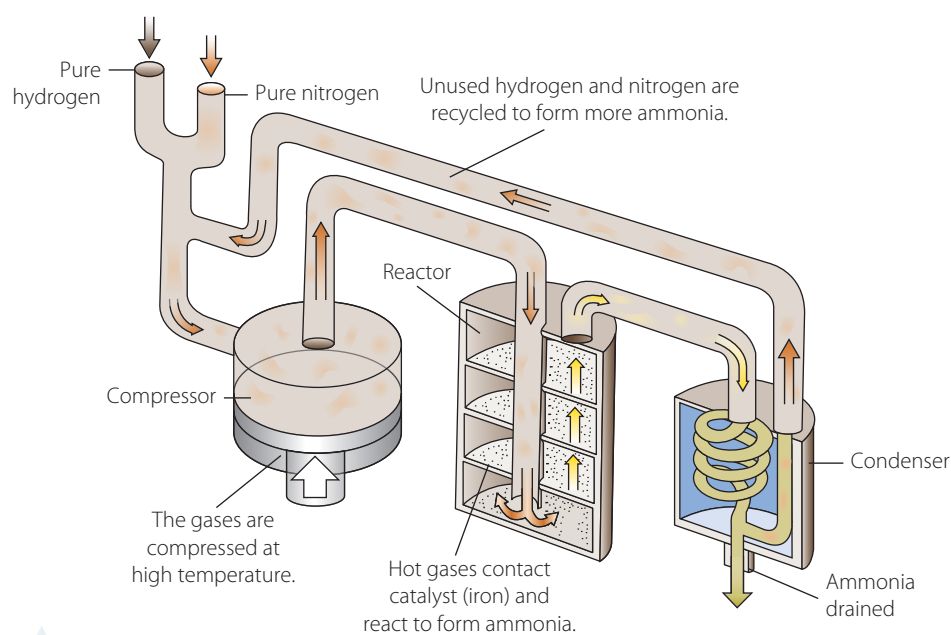
FIGURE 16.12 The industrial production of ammonia
