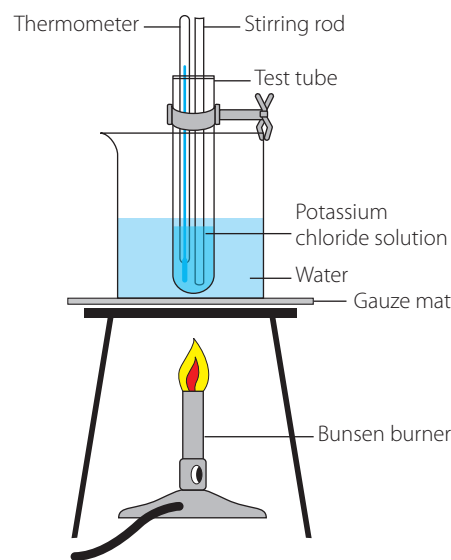
FIGURE 4.10 Experimental set-up for determination of a solubility curve
