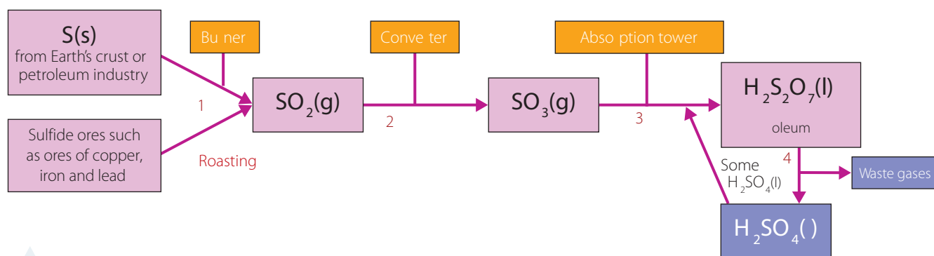
FIGURE 16.10 Stages of sulfuric acid production
