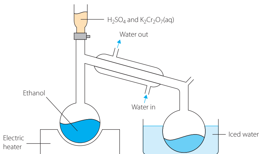
FIGURE 11.4 Collection of aldehyde through distillation
