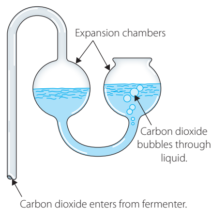
FIGURE 11.8 A simple airlock used to exclude oxygen from a fermentation mixture
