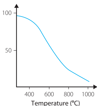
FIGURE 16.11 Yield of sulfur trioxide as temperature changes
