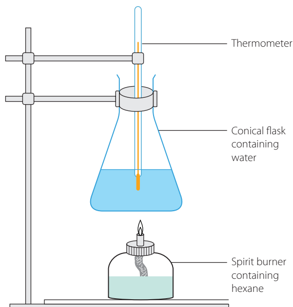
FIGURE 11.2 Equipment set-up to measure the enthalpy of combustion of a fuel
