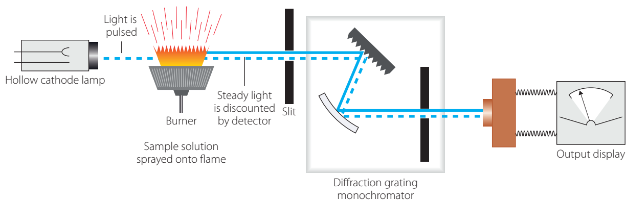
FIGURE 14.13 The process of atomic absorption spectroscopy
