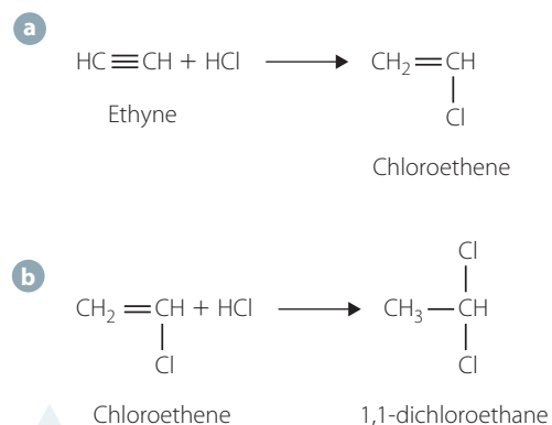
FIGURE 10.8 Addition of hydrogen chloride to a ethyne and b chloroethene
