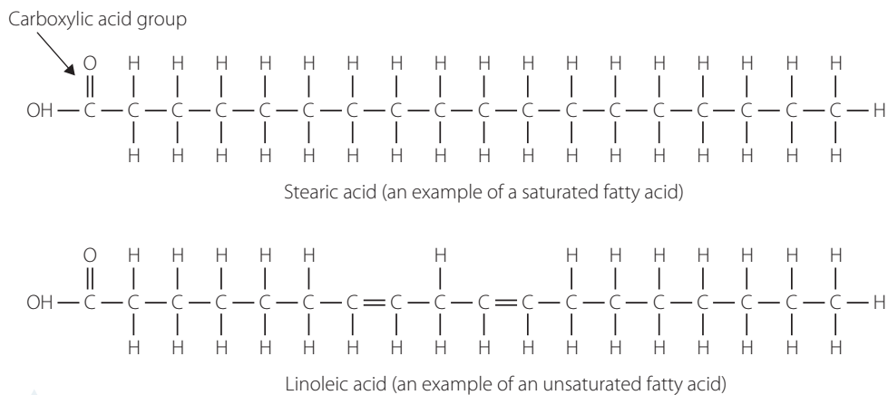
FIGURE 11.11 Examples of saturated and unsaturated fatty acids
