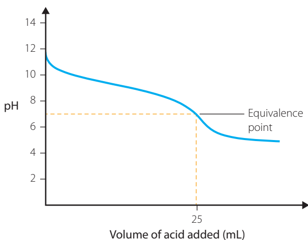
FIGURE 7.10 A pH graph for a titration involving a weak base and a weak acid
