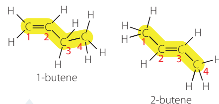
FIGURE 8.10 The different possible positions for the double bond in a butene molecule
