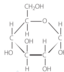
FIGURE 9.6 Glucose molecule with multiple hydroxyl groups
