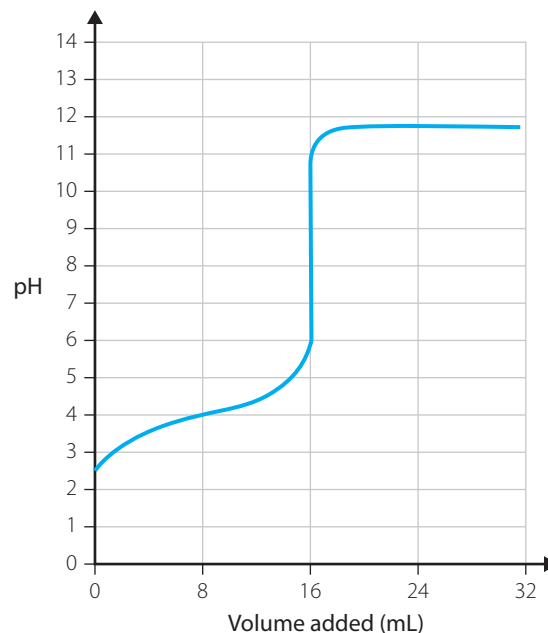
FIGURE 7.23 A pH curve for a titration
