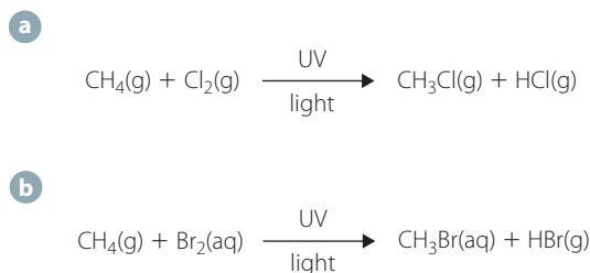
FIGURE 10.12 Addition of chlorine and bromine to methane under UV light
