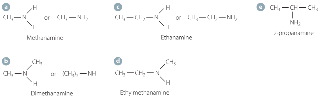
FIGURE 9.14 Some simple amines
