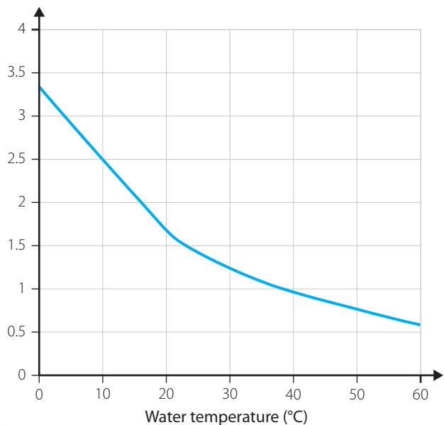
FIGURE 10.17 The effect of temperature on the solubility of carbon dioxide
