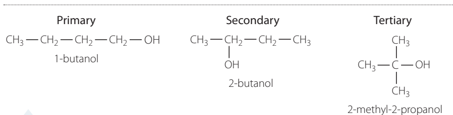
FIGURE 9.4 Primary, secondary and tertiary alcohols
