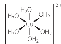
FIGURE 14.8 Hexaaquacopper(II)
