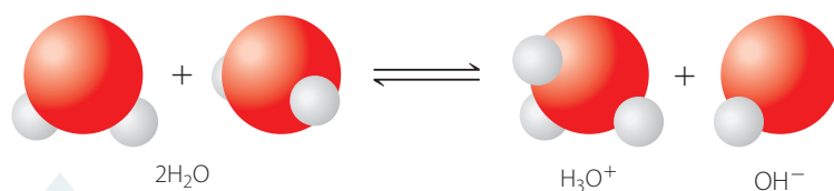
FIGURE 6.11 Water reacts with itself in an equilibrium reaction to form hydronium and hydroxide ions, showing water's amphoteric nature.
