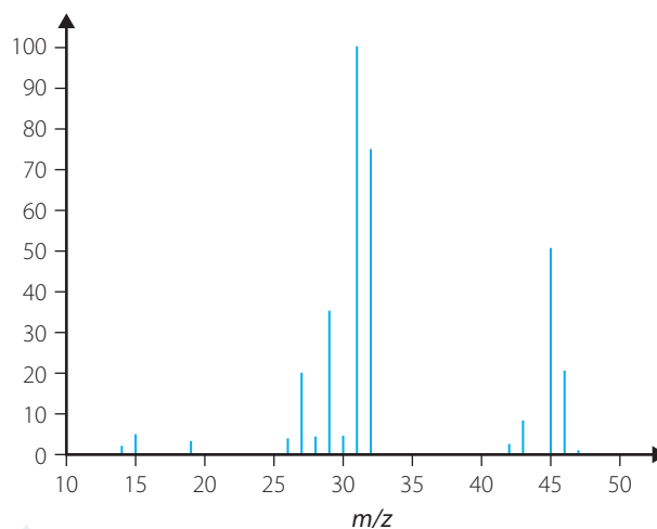
FIGURE 15.10 Mass spectrum of contaminated sample
