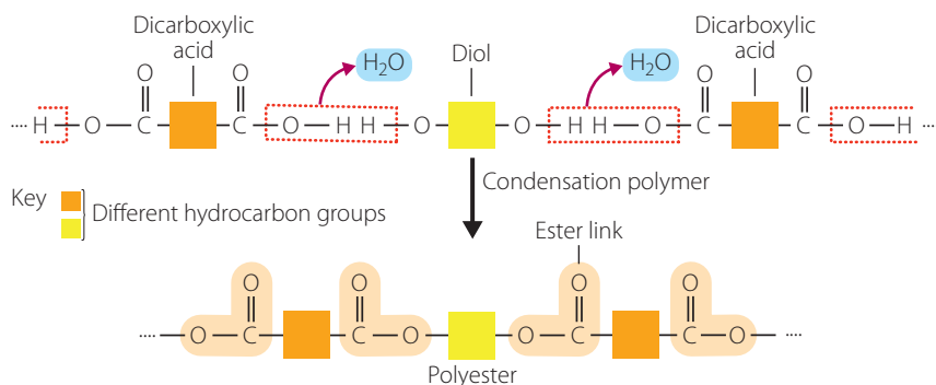
FIGURE 13.15 The formation of a polyester from a diol monomer and a dicarboxylic acid monomer
