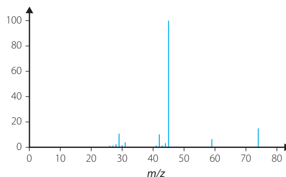
FIGURE 15.33 Mass spectrum of compound X
