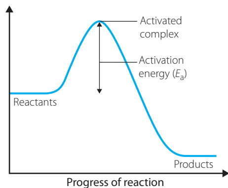
FIGURE 2.7 Activation energy of a reaction
