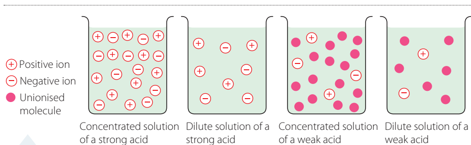
FIGURE 6.10 Concentrated and dilute solutions of a weak and strong acid
