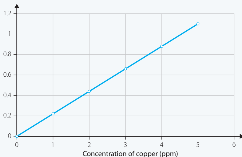
FIGURE 14.14 Calibration curve for determination of copper concentration
