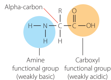
FIGURE 13.20 General structure of an alpha amino acid
