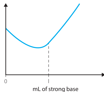
FIGURE 7.13 Conductivity graph for a titration involving a weak acid and a strong base
