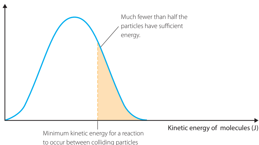
FIGURE 2.8 The number of particles with enough energy for a successful collision
