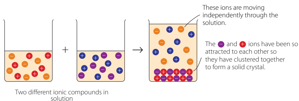
FIGURE 4.16 Explaining the formation of silver chloride precipitate ( Note: This is a simplified model of the association process.)
