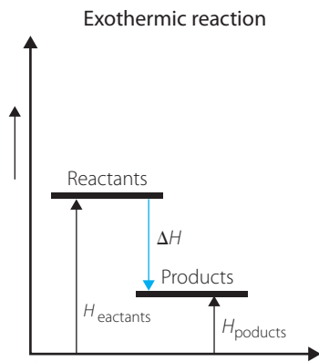
FIGURE 5.6 In an exothermic reaction, energy is released since energy of reactants is greater than energy of products.
