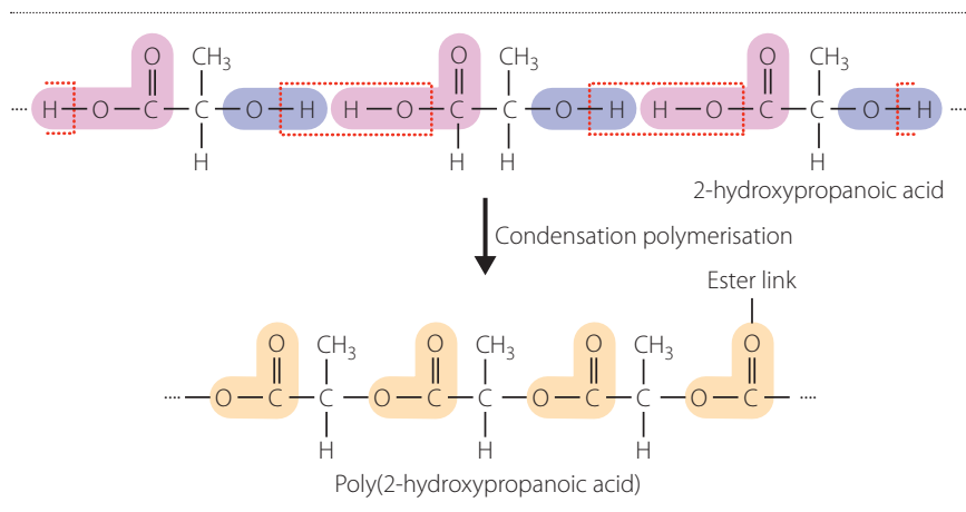
FIGURE 13.14 The formation of a polyester from a single monomer (2-hydroxypropanoic acid)
