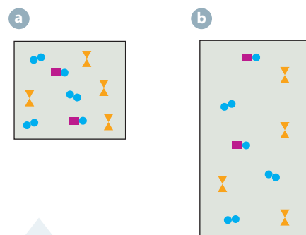
FIGURE 2.16 a Gaseous molecules of reactants and products in a particular volume b gaseous molecules of reactants and products when volume of system has been doubled
