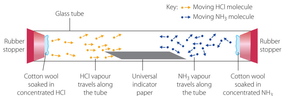
FIGURE 5.11 The reaction between ammonia gas and hydrogen chloride gas
