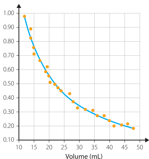
FIGURE 1.9 A pressure–volume graph for a gas needs a large number of data points to show the hyperbola shape.
