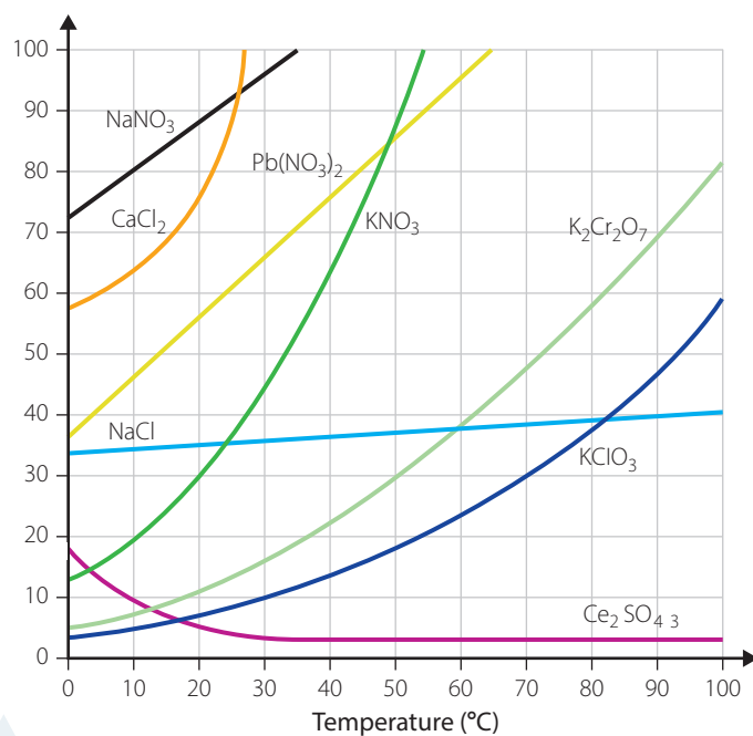
FIGURE 4.8 A selection of solubility curves for various salts
