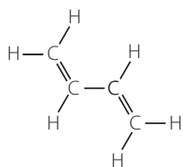
FIGURE 13.10 Butadiene monomer
