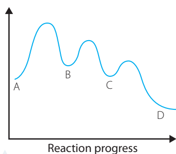
FIGURE 16.6 Energy profile diagram for a multistep reaction
