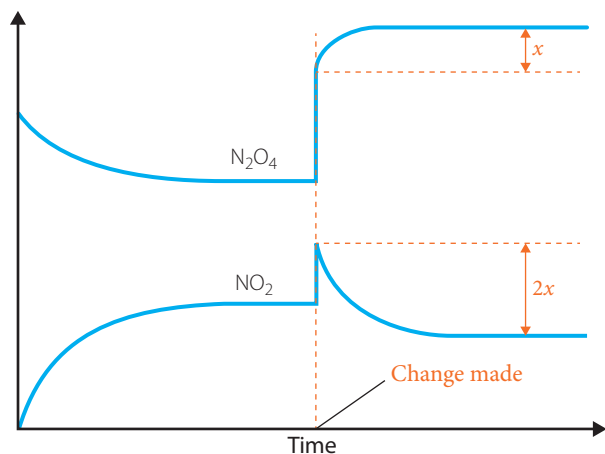
FIGURE 2.23 Concentration of \text{N}_2\text{O}_4 and \text{NO}_2 over time
