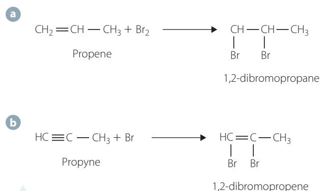
FIGURE 10.7 Addition of bromine to a propene and b propyne
