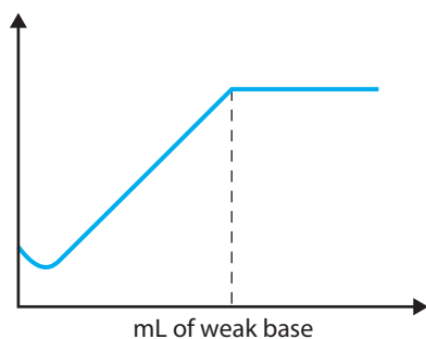
FIGURE 7.14 Conductivity graph for a titration involving a weak acid and a weak base
