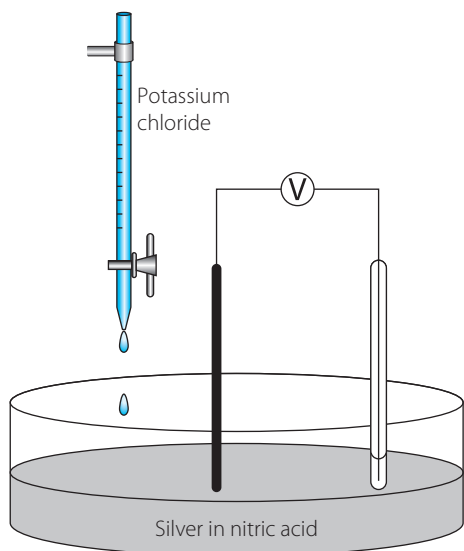
FIGURE 7.19 Set-up for a potentiometric titration
