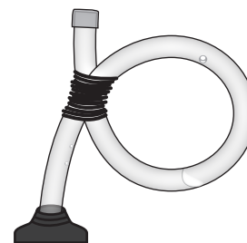
FIGURE 11.9 A simple airlock can be made from a plastic hose partially filled with water.
