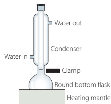
FIGURE 12.7 Apparatus used for refluxing an ester mixture
