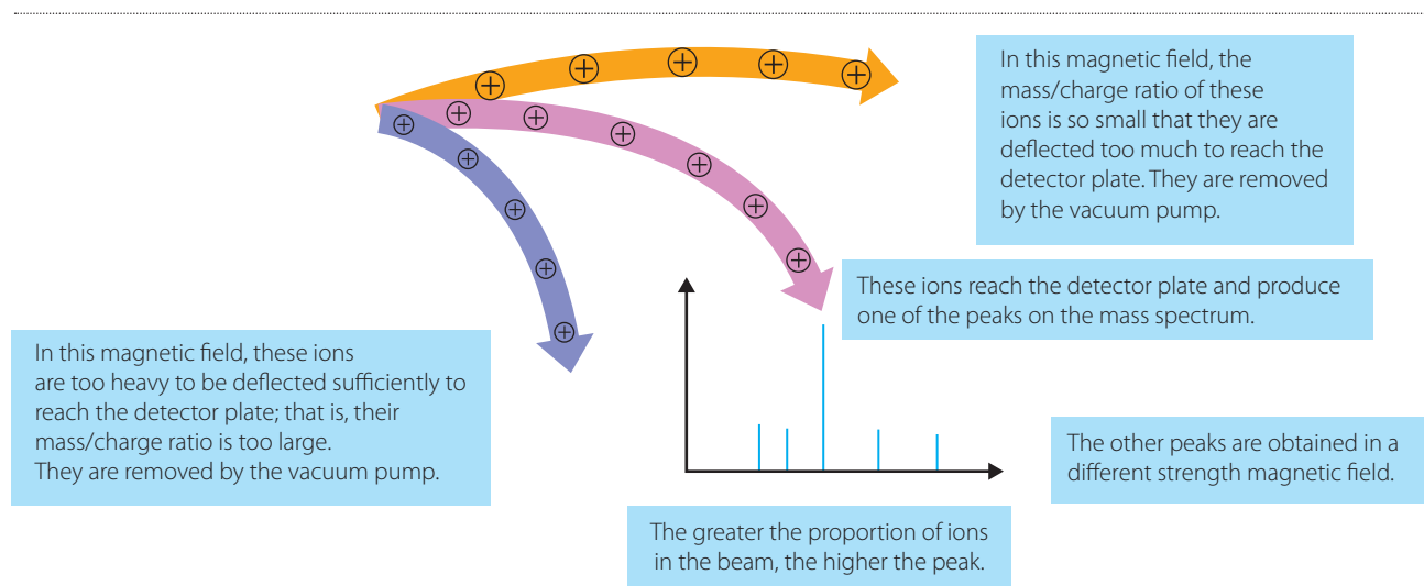
FIGURE 15.5 Focusing and collecting an ion stream
