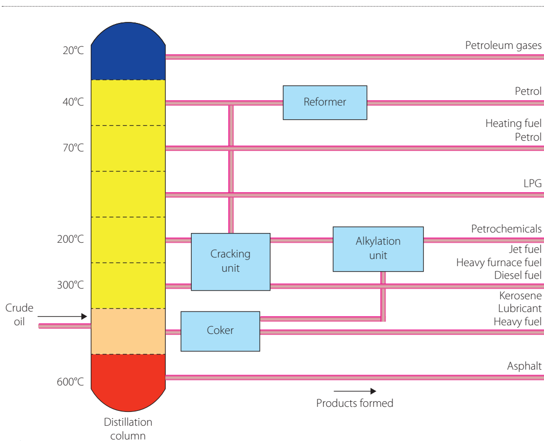
FIGURE 10.13 Distillation column in an oil refinery
