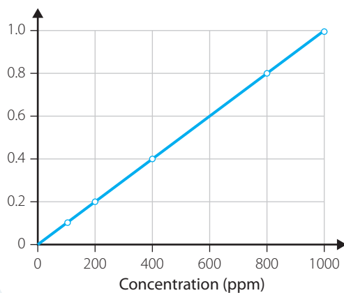
FIGURE 14.16 A typical calibration curve for copper(II) tetrammine ions at 610 nm
