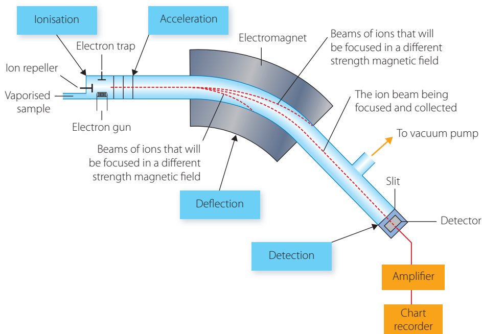
FIGURE 15.3 The mass spectrometer – a schematic diagram
