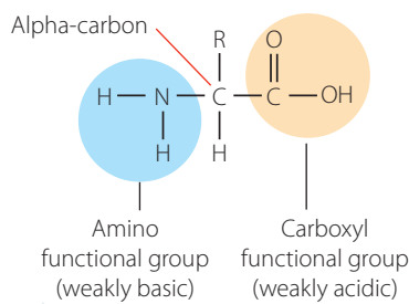
FIGURE 12.11 Amino acids contain an organic acid and an organic base in the same molecule.
