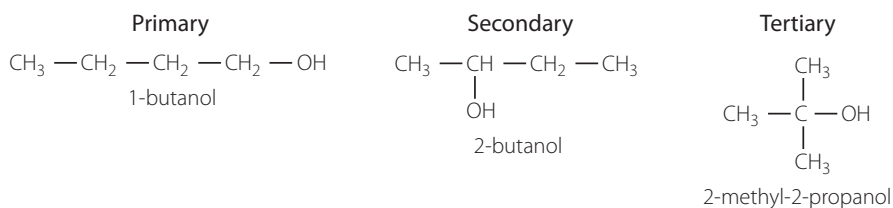
FIGURE 11.3 Primary, secondary and tertiary alcohols
