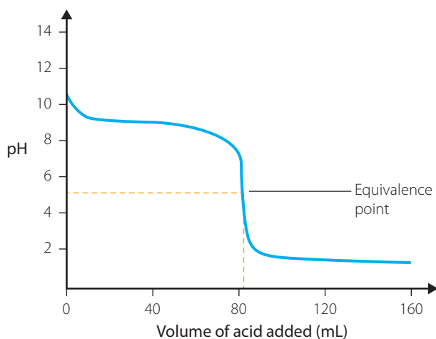
FIGURE 7.9 A pH graph for a titration involving a weak base and a strong acid
