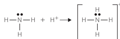
FIGURE 14.7 Example of the formation of a coordinate covalent bond
