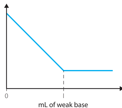
FIGURE 7.12 Conductivity graph for a titration involving a strong acid and a weak base
