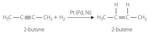
FIGURE 10.6 Reaction of 2-butyne to form 2-butene with a Lindlar catalyst
