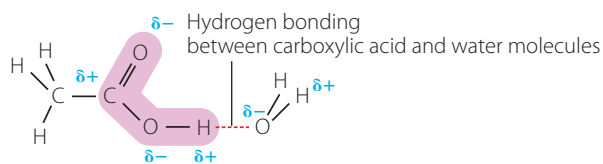
FIGURE 9.10 Carboxylic acids form hydrogen bonds with water.
