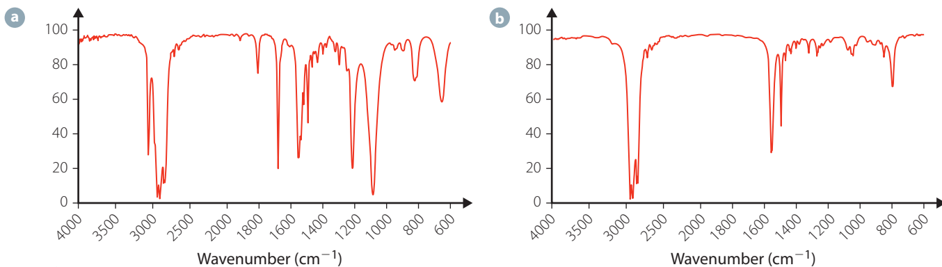
FIGURE 15.31 1-hexene or hexane spectra (in no particular order)
