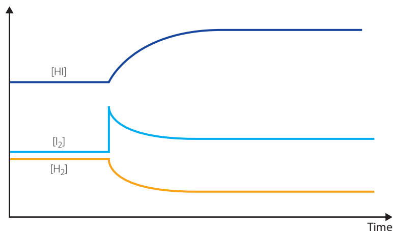
FIGURE 2.15 Concentrations of reactants and product following a change in concentration for the reaction: \text{H}_2(\text{g}) + \text{I}_2(\text{g}) \rightleftharpoons 2\text{HI}(\text{g})
