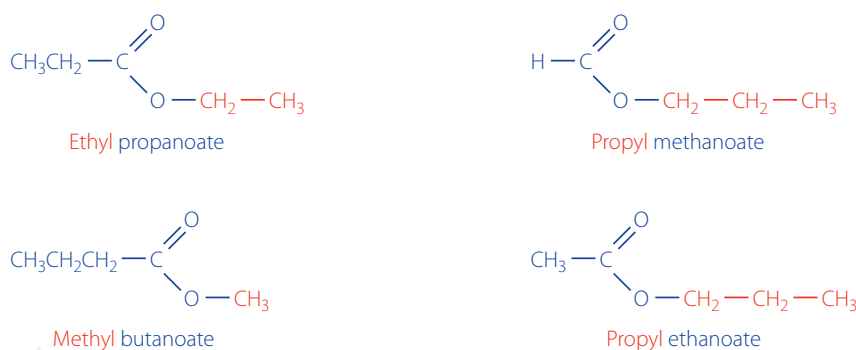
FIGURE 12.5 Naming esters through their structure
