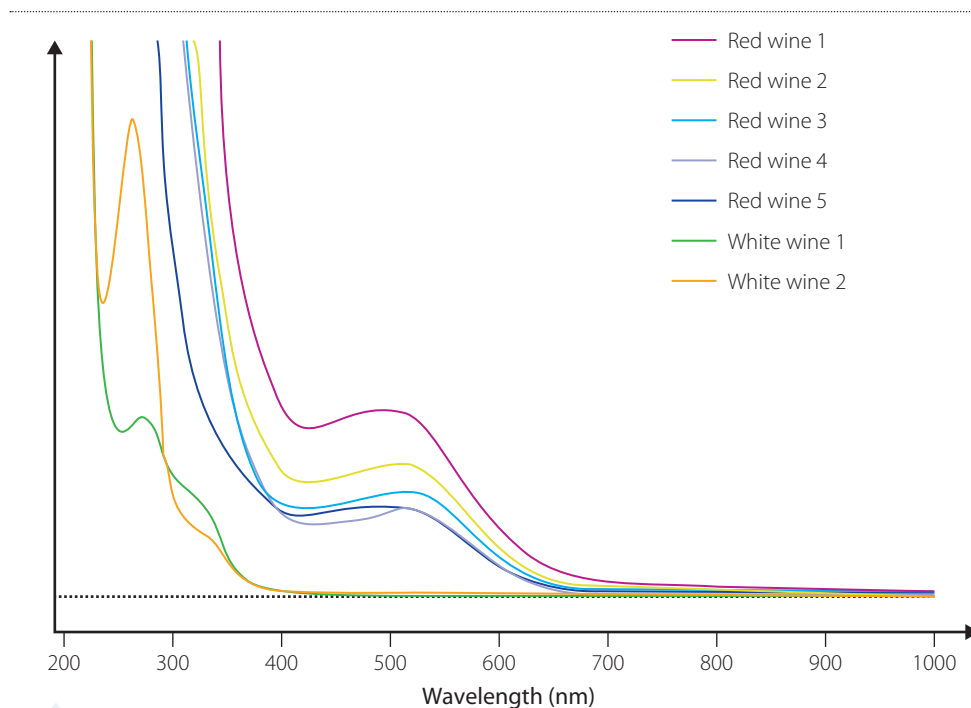
FIGURE 15.29 Absorbance spectra of wine samples
