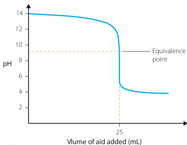
FIGURE 7.8 A pH graph for a titration involving a strong base and a weak acid
