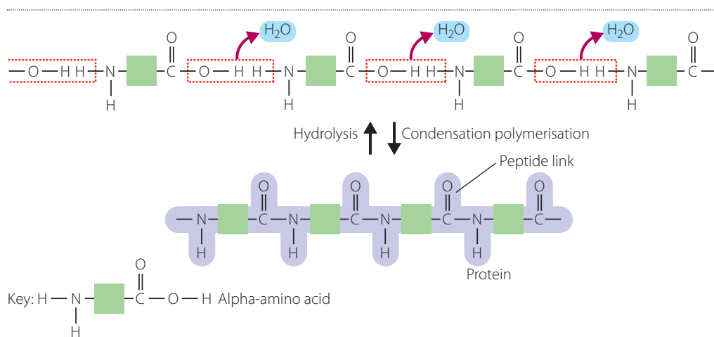
FIGURE 13.22 Forming a polypeptide and breaking it down again
