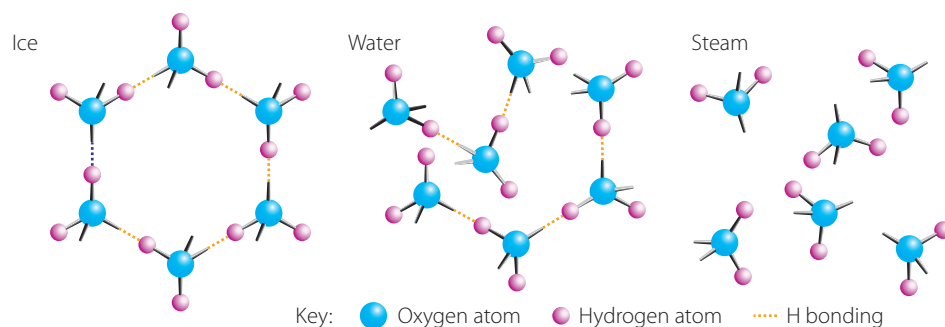
FIGURE 4.4 The structure of ice compared to that of liquid water and steam, showing hydrogen bonding
