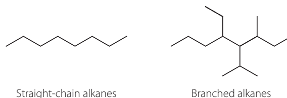
FIGURE 8.8 Straight-chain and branched alkanes
