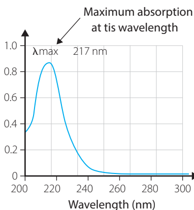
FIGURE 15.28 UV–vis spectrum for 1,3-butadiene
