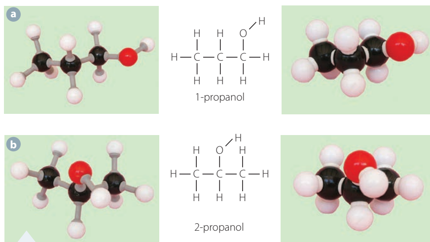
FIGURE 9.3 Ball and stick, structural and space-filling models for a 1-propanol and b 2-propanol
