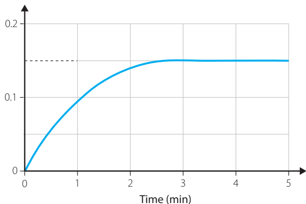
FIGURE 3.5 Quantitative equilibria
