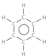
FIGURE 8.3 The basic structure of benzene
