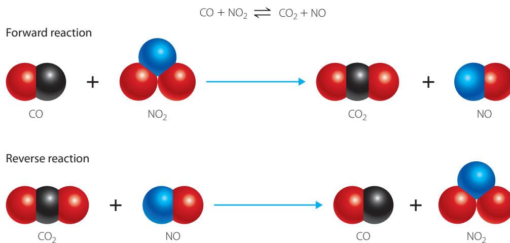
FIGURE 2.6 Forward and reverse reactions
