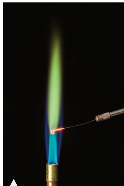
FIGURE 14.5 The flame colour produced by barium
