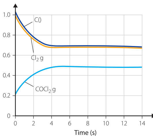
FIGURE 2.14 Concentrations of various chemical species over time
