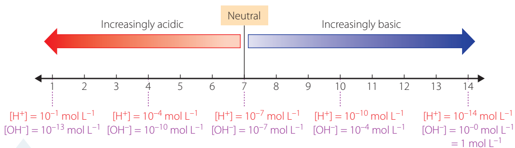
FIGURE 6.13 The pH scale
