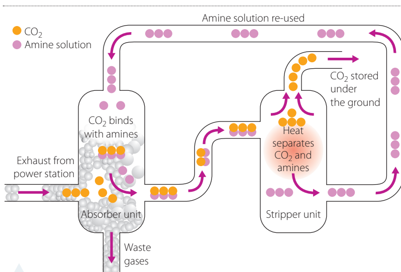
FIGURE 10.18 Process of post-combustion carbon capture
