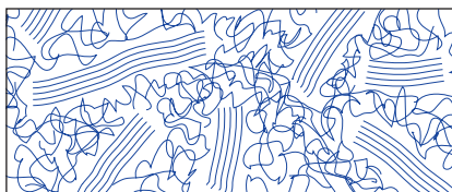
FIGURE 13.12 Crystalline and amorphous regions in a polymer
