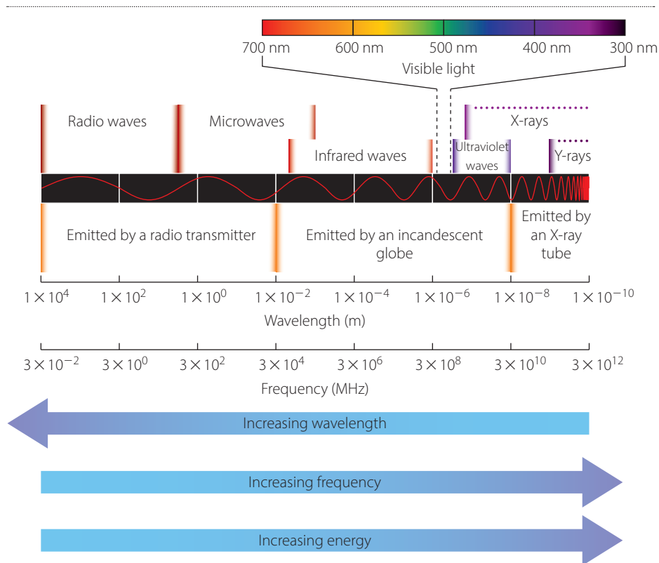
FIGURE 15.2 The electromagnetic spectrum ( Note: The wavelength of the waves that make up visible light is so small that it is recorded in nanometres, nm ( 1 \text{ nm} = 10^{-9} \text{ m} ). The frequency of the waves has been measured in megahertz, MHz ( 1 \text{ MHz} = 10^6 \text{ Hz} ).
