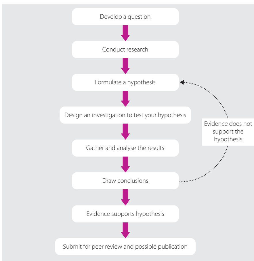
FIGURE 1.2 Diagrammatic representation of the scientific method
