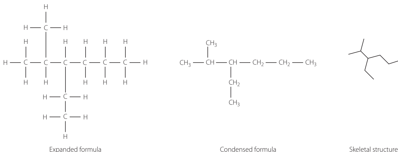
FIGURE 8.5 Expanded formula, condensed formula and skeletal structure representations of organic molecules
