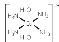
FIGURE 14.9 Diaquatetraamminecopper(II)
