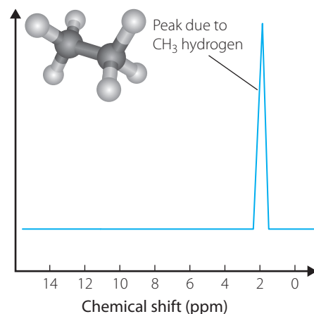
FIGURE 15.16 The low-resolution ^1\text{H} NMR spectrum of ethane ( \text{CH}_3\text{CH}_3 )
