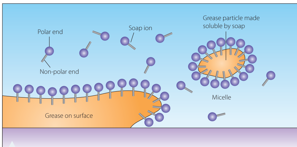
FIGURE 12.17 The cleaning action of soap
