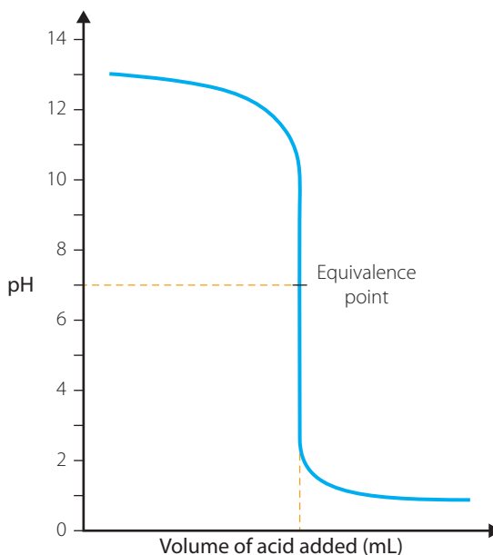
FIGURE 7.7 A pH graph for a titration involving a strong base and a strong acid
