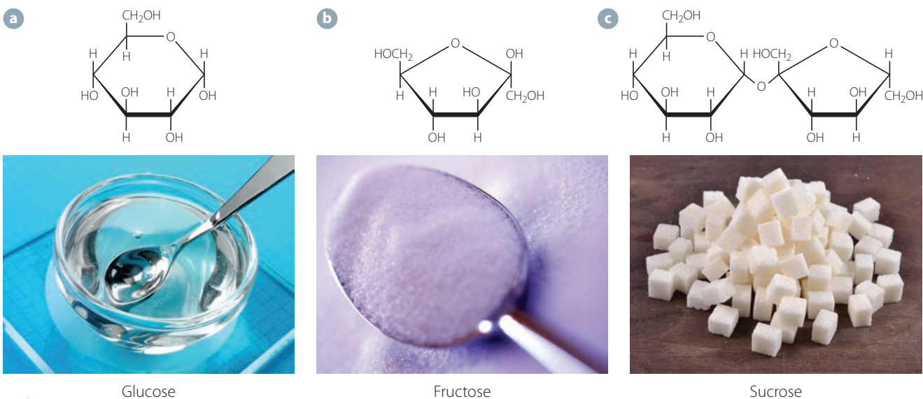
FIGURE 11.6 Chemical structures and appearance of a glucose, b fructose and c sucrose
