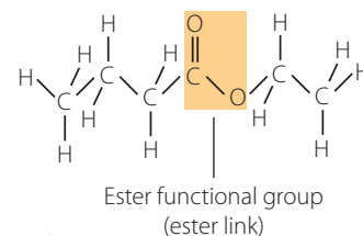
FIGURE 12.3 The ester, ethyl butanoate
