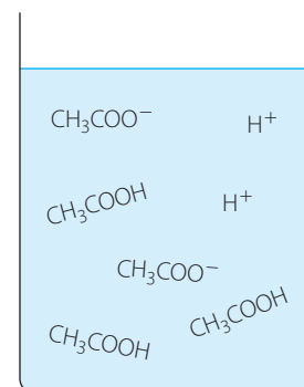
FIGURE 3.2 In simplified form, acetic acid only partially ionises to form hydrogen ions and acetate ions.
