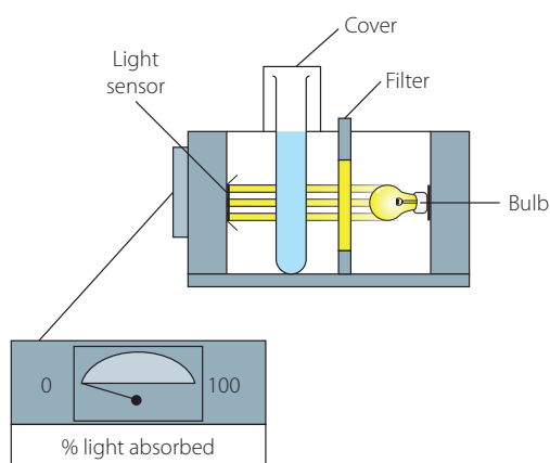
FIGURE 14.15 The process by which a colourimeter works
