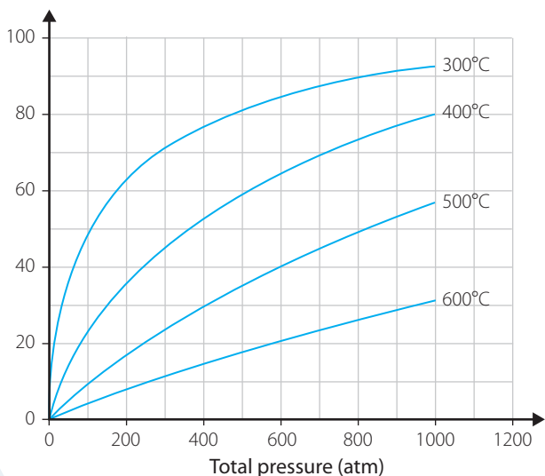
FIGURE 16.13 Production of ammonia at different temperatures and pressures
