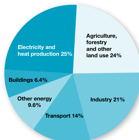
Figure 12.4 – Sources of greenhouse gas emissions
