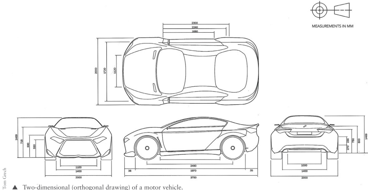
▲ Two-dimensional (orthogonal drawing) of a motor vehicle.
