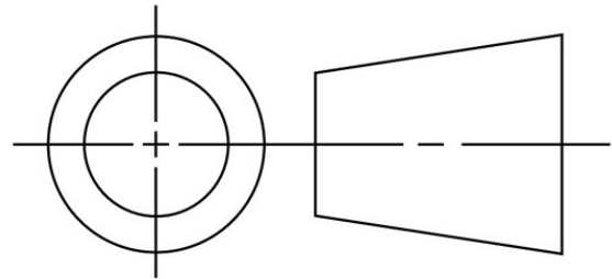
▲ The third-angle projection symbol. This should appear on all third-angle orthogonal drawings. Refer to the VCAA Technical Drawing Specifications for advised proportions when creating this symbol.
