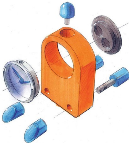
▲ Exploded isometric view of an alarm clock
