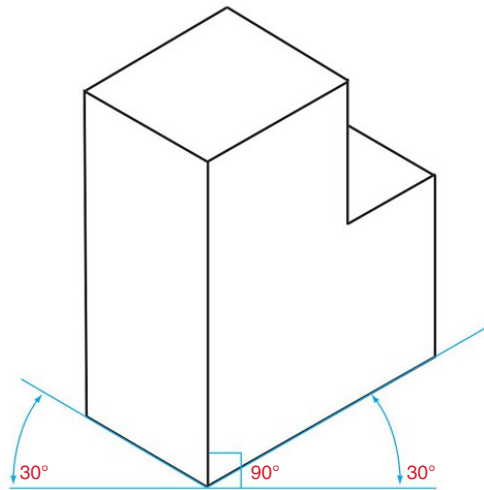
▲ Isometric drawing
