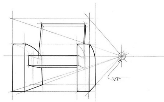
▲ One-point perspective drawing of club armchair using crating method
