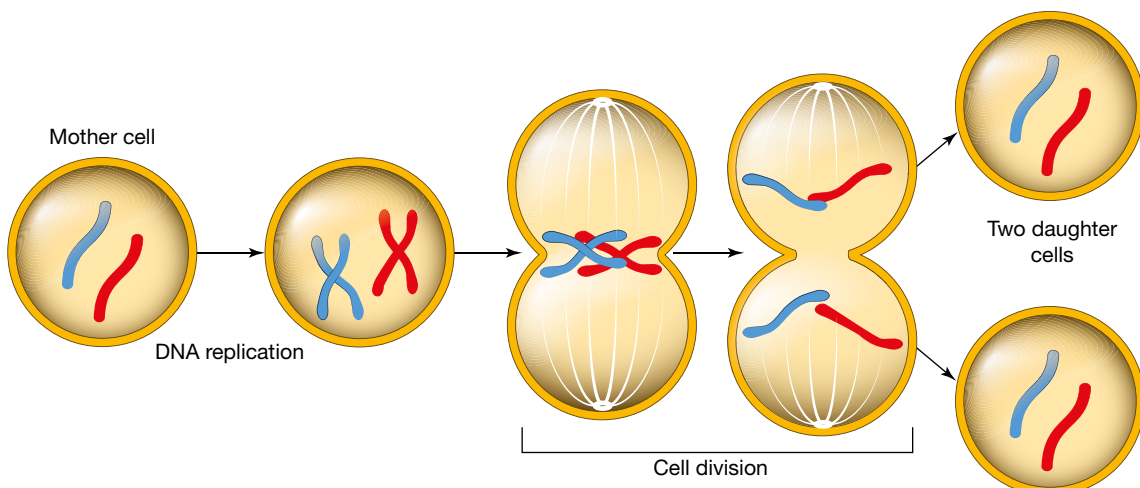
FIGURE 2.62 Mitosis results in the production of identical daughter cells
