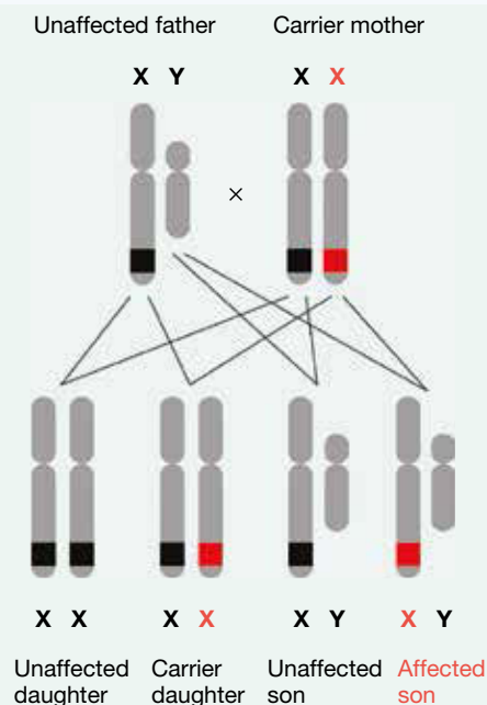
FIGURE 2.94 The inheritance of haemophilia. The allele for haemophilia is shown in red.
