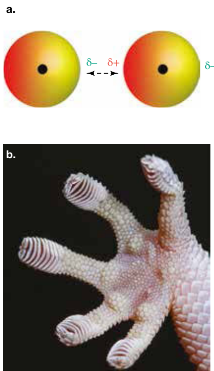
FIGURE 9.24 a. Van der Waals forces and b. the setae and spatulae of gecko's feet
