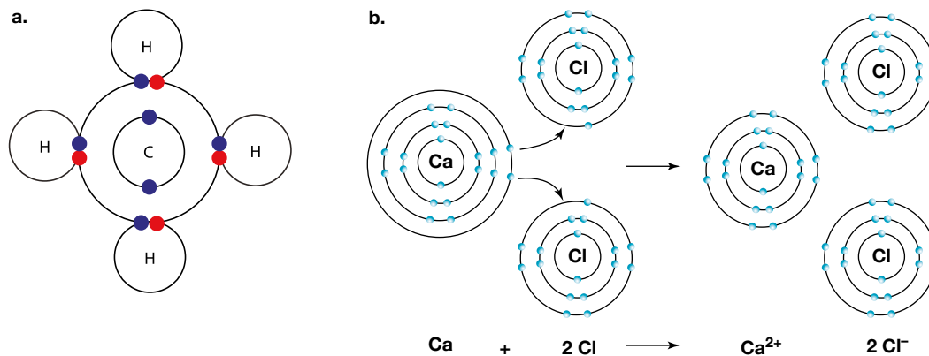
FIGURE 4.37 a. A molecule of methane with covalent bonding b. Ionic bonding in calcium chloride
