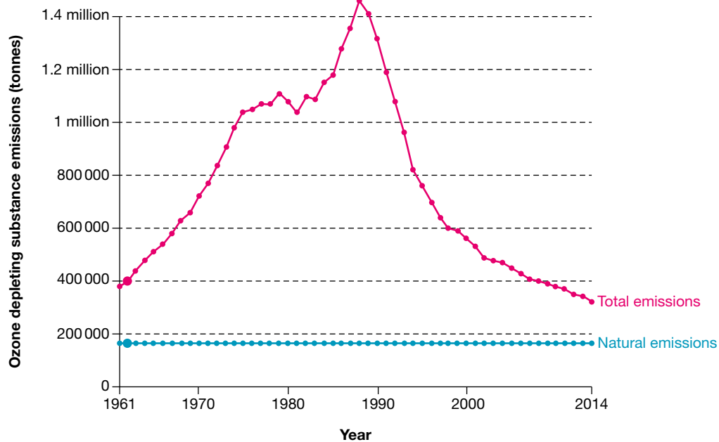
FIGURE 7.36 Ozone depleting substance emissions since 1961
