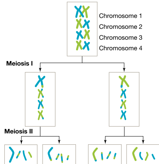
FIGURE 3.14 Independent assortment and crossing over during meiosis are two causes of variation.
