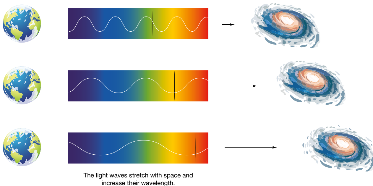
FIGURE 6.14 Expansion of space explains redshift. Any light waves passing through the expanding space increase their wavelengths and become more 'red'.
