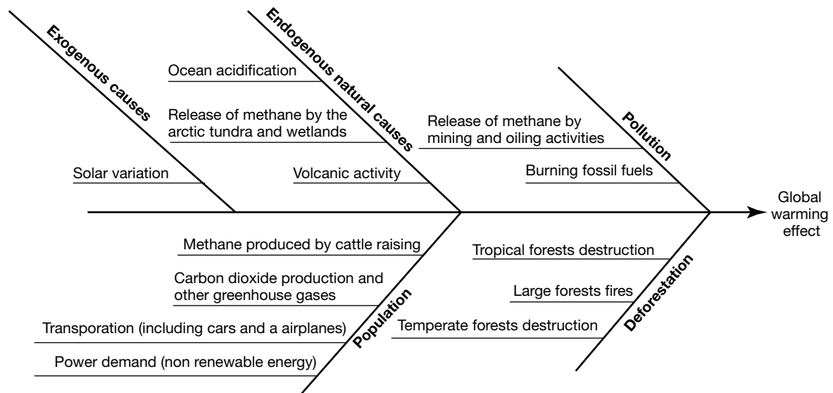
FIGURE 7.69 A fishbone diagram showing causes of global warming
