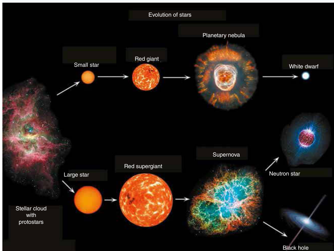
FIGURE 6.11 Large stars follow a different evolutionary sequence to smaller stars like the Sun.
