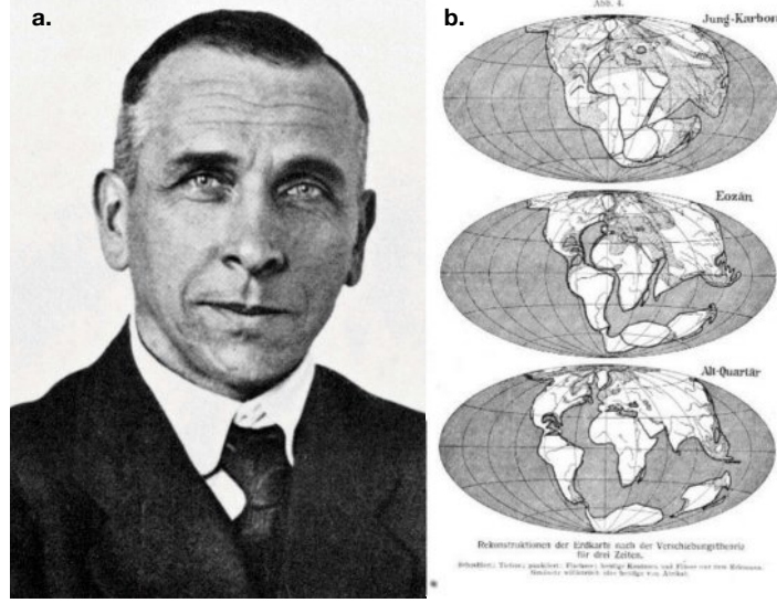
FIGURE 3.54 a. Alfred Wegener (1880–1930) b. Wegener's earliest maps showing continental drift
