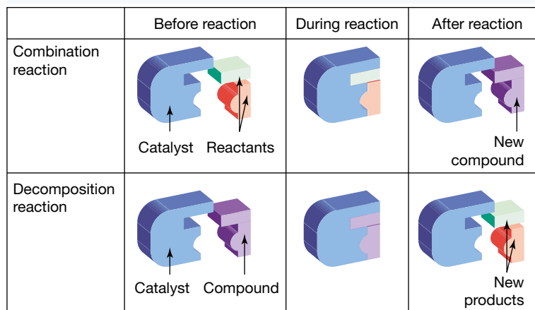
FIGURE 5.37 How catalysts work
