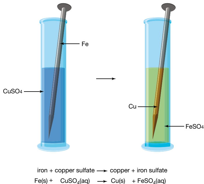
FIGURE 4.35 The displacement reaction involving a metal and metal salt
