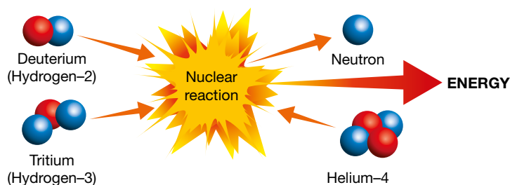
FIGURE 6.7 This nuclear fusion reaction in stars releases vast amounts of energy.
