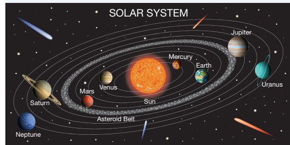
FIGURE 9.53 Travelling to Mars relies on it being closer to Earth in orbit
