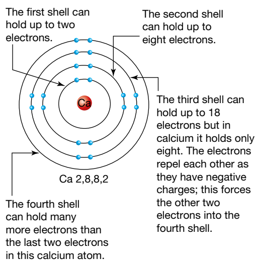
FIGURE 4.18 A calcium atom has 20 electrons.
