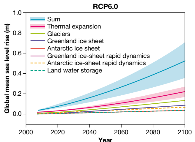
FIGURE 7.55 Projected sea level rise for a scenario where the greenhouse emission rate is high but is stabilised by 2100 using a range of technologies and strategies to reduce the emission rate
