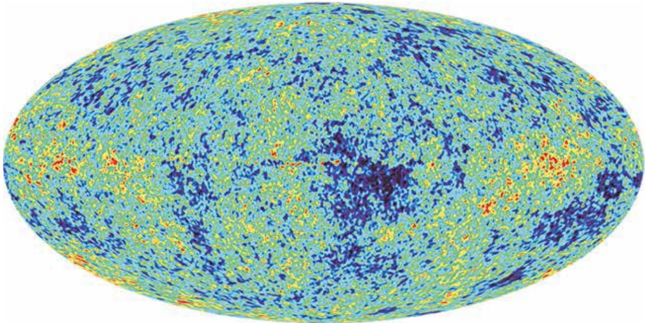
FIGURE 6.18 WMAP image of cosmic microwave background radiation
