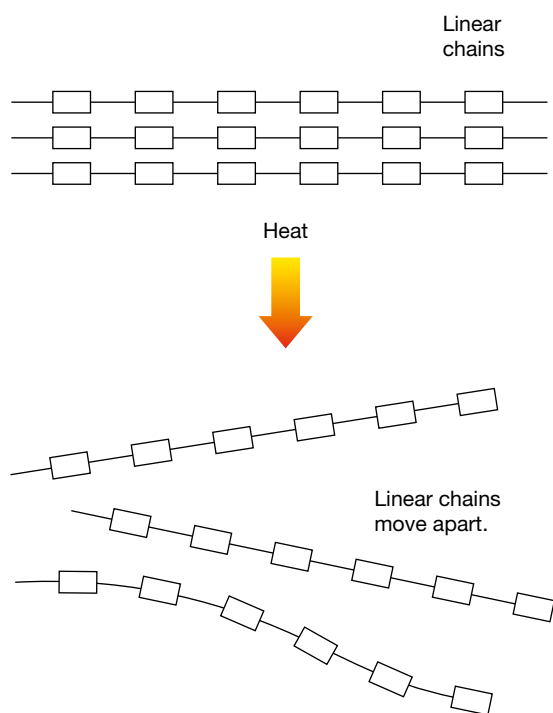
FIGURE 5.35 Structure of a thermoplastic polymer. The chains of monomer molecules are able to slide past one another when the polymer is heated.
