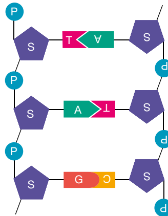
FIGURE 2.30 DNA forming a double stranded molecule
