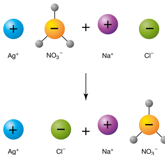
FIGURE 5.10 Ions can change partners when a chemical reaction takes place.
