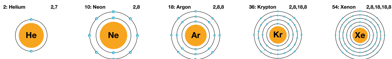
FIGURE 4.22 The full outer shells of the noble gases
