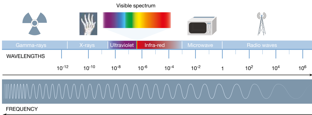
FIGURE 6.21 The electromagnetic spectrum.
