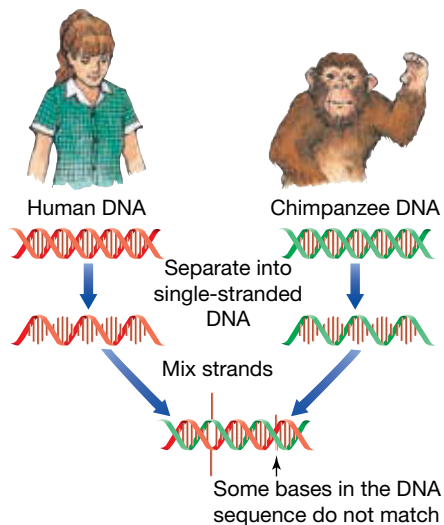
FIGURE 3.81 The process involved in DNA hybridisation.
