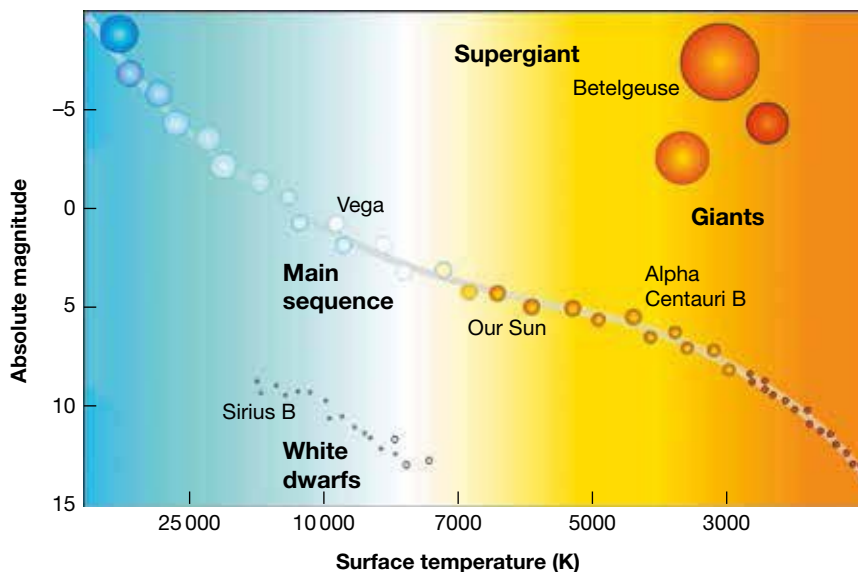
FIGURE 6.9 The Hertzsprung–Russell diagram sorts stars according to their absolute magnitude (or luminosity) and surface temperature.
