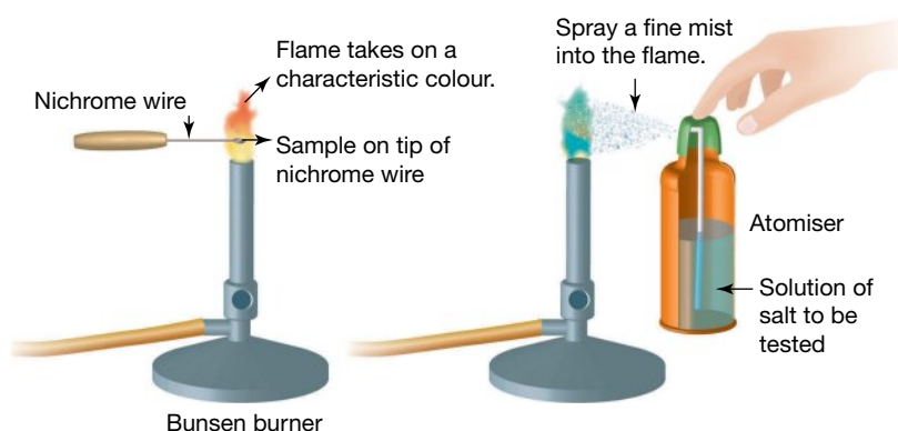
FIGURE 4.21 Various metal ions produce characteristic colours when they are volatilised in a flame.
