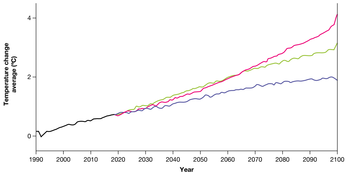
FIGURE 7.39 Earth's temperature change prediction in 2100. The black line represents an average of a set of temperatures. The coloured lines represent average expected temperatures under three emissions scenarios that may occur in the future. These scenarios are as follows. Humans worldwide make more sustainable choices and use renewable energy (purple), a balance is achieved between use of fossil fuels and renewable sources (green), and humans continue to accelerate carbon emissions (pink).
