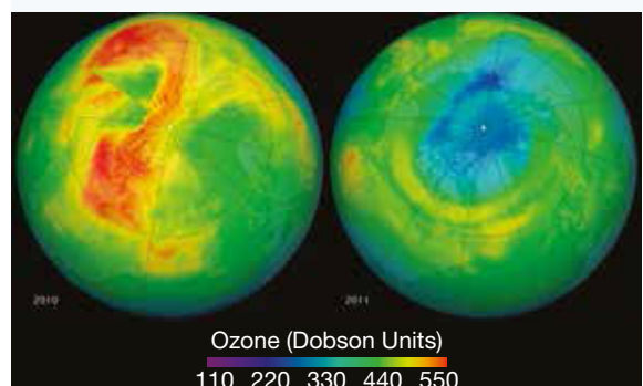
FIGURE 7.33 Ozone concentrations over the Arctic, 19 March 2010 (L) and 19 March 2011 (R). In 2010, a high concentration of ozone can be seen, compared to a low concentration in 2011.
