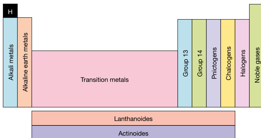
FIGURE 4.8 The named families of elements in the periodic table
