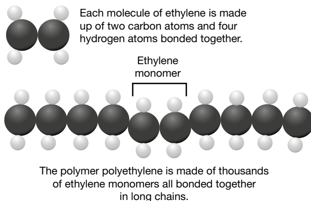
FIGURE 5.29 A polymer is made up of smaller units called monomers bonded together.
