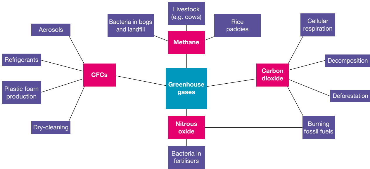
FIGURE 7.26 Some sources of greenhouse gases
