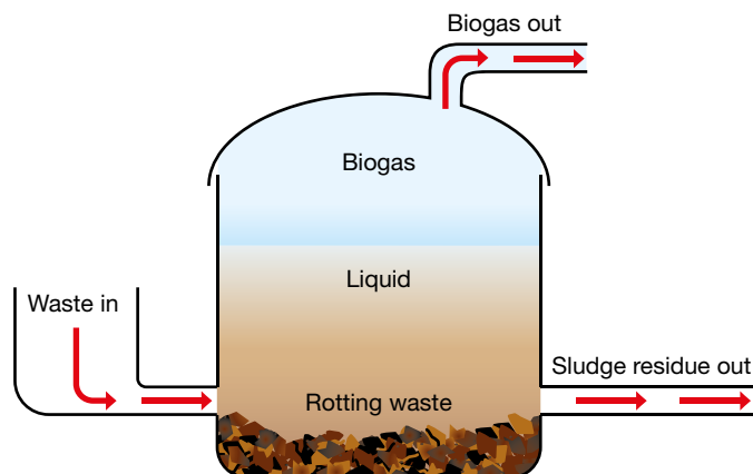
FIGURE 5.27 A simple household biogas digester
