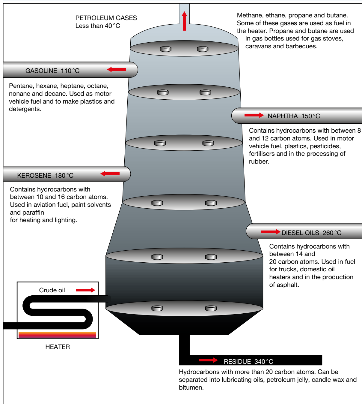
FIGURE 5.25 The fractional distillation of crude oil
