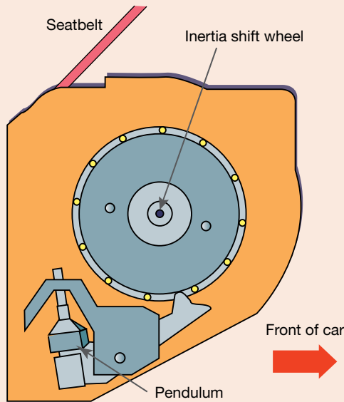
FIGURE 8.34 This inertia reel seatbelt is shown in the locked position. If rapid deceleration occurs, the small pendulum is able to swing forward with the inertia of the vehicle and lock the reel holding the seatbelt, preventing the passenger from moving forward.
