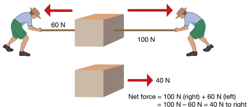
FIGURE 8.19 Net forces can be calculated when forces are unbalanced using sign and direction convention.
