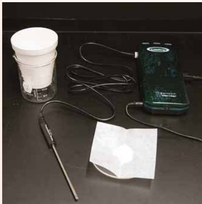
FIGURE 1.40 The equipment required for citric acid and baking soda
