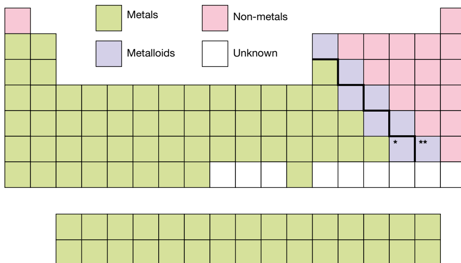
FIGURE 4.9 The periodic table can be broken into metals, non-metals and metalloids. Polonium (*) and astatine (**) are sometimes disputed as being metalloids.
