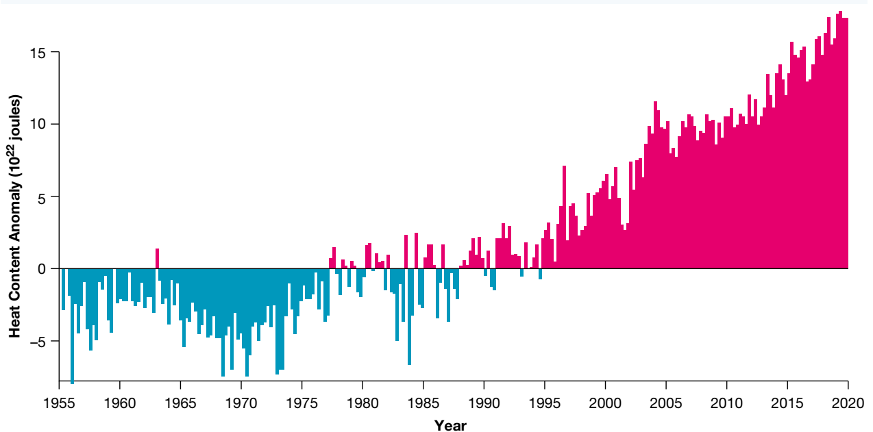
FIGURE 7.22 Changes in the long-term average global ocean heat content, 1955 to 2020
