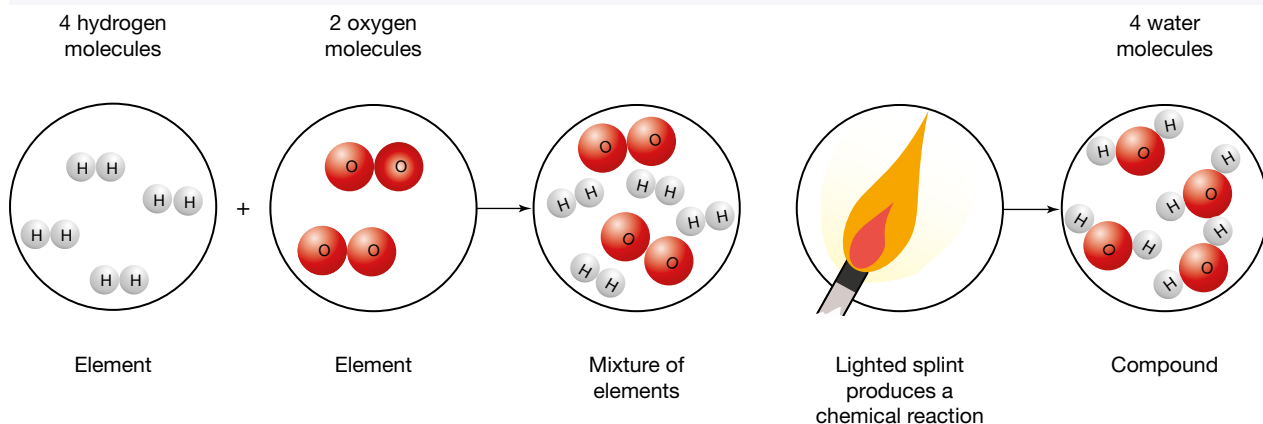
FIGURE 5.5 The chemical reaction between oxygen and hydrogen
