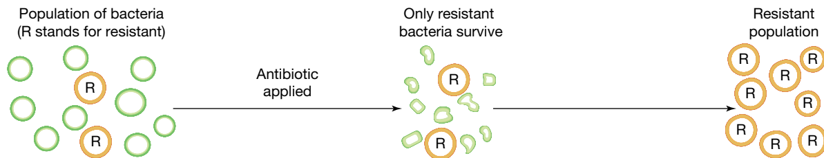
FIGURE 3.37 Mutations in bacteria can result in some individuals having resistance against antibiotics. When these bacteria reproduce, their offspring also show antibiotic resistance.
