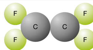
FIGURE 5.32 A tetrafluoroethene molecule; this is the monomer from which teflon is formed.
