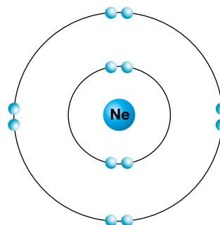
FIGURE 4.15 An electron shell diagram
