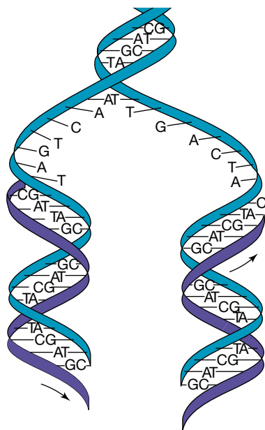
FIGURE 2.43 DNA replication is semi-conservative — a combination of original (blue) and new (purple) strands.
