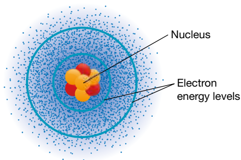
FIGURE 4.14 An atom containing a cloud of electrons arranged into energy levels or shells.
