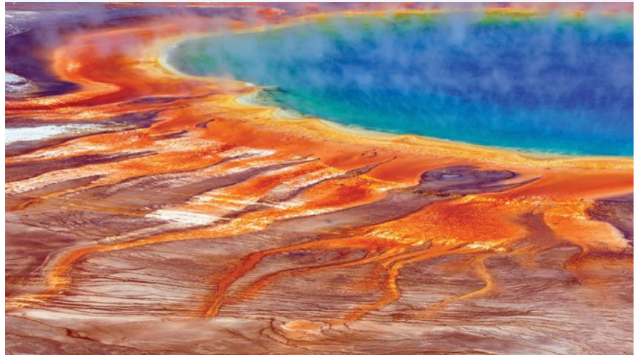
FIGURE 7.70 Grand Prismatic Spring in Yellowstone National Park
