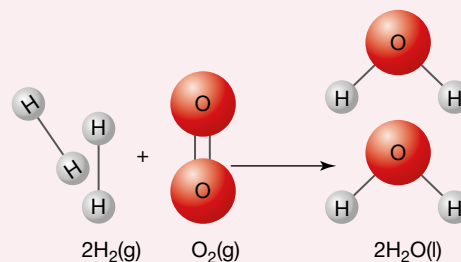
FIGURE 5.7 Checking reactants and products balance
