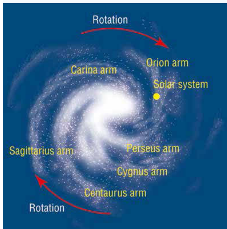
FIGURE 6.12 The Milky Way galaxy
