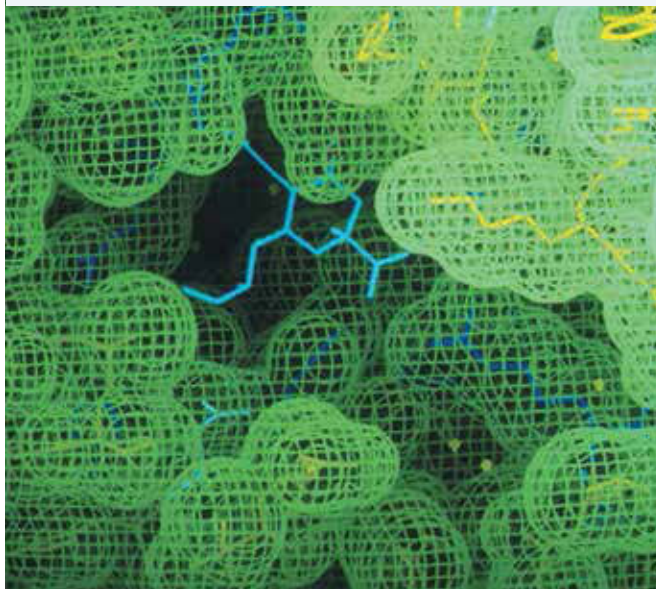
FIGURE 11.48 Images of complex structures like this helped develop the influenza-fighting drug Relenza™. The synchrotron can also be used to develop anti-toxins.
