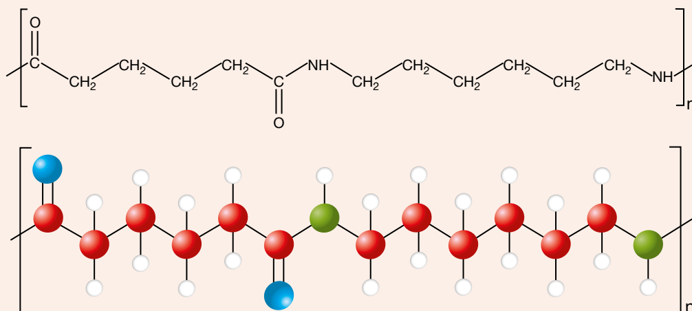
FIGURE 5.31 Nylon is a co-polymer.
