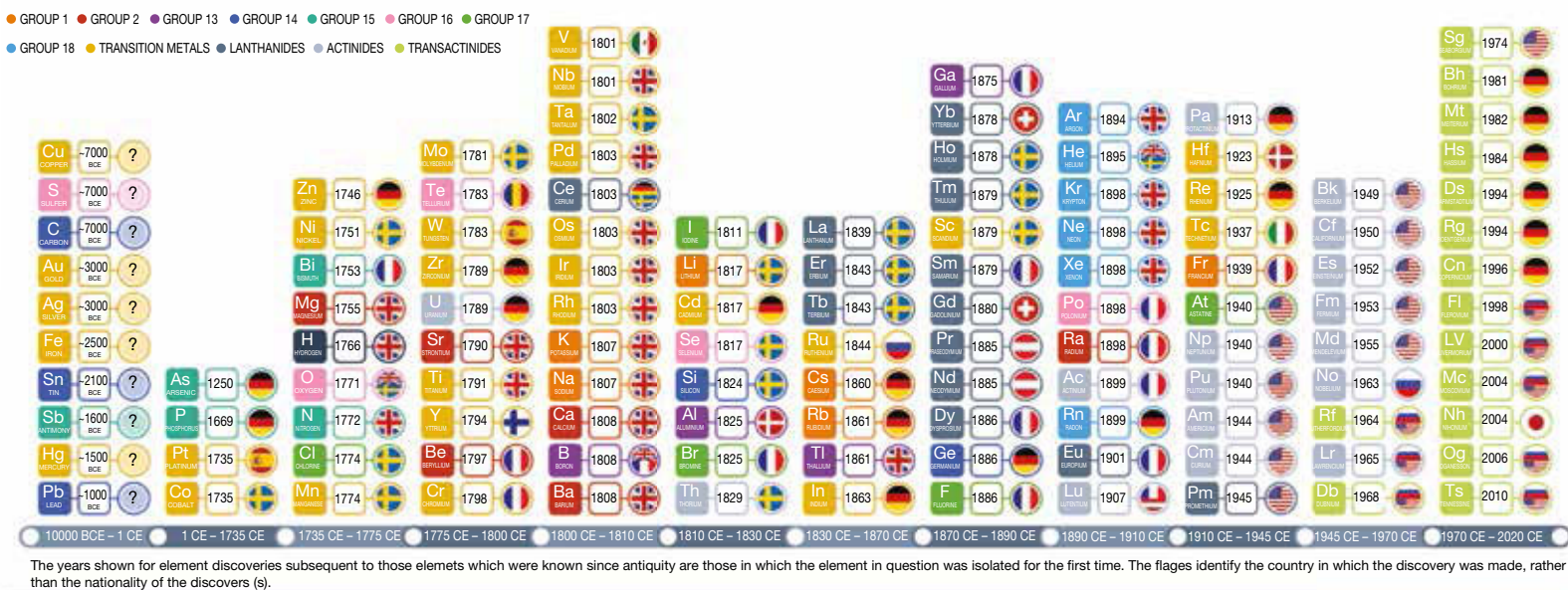
FIGURE 4.3 A timeline of the discovery of elements
