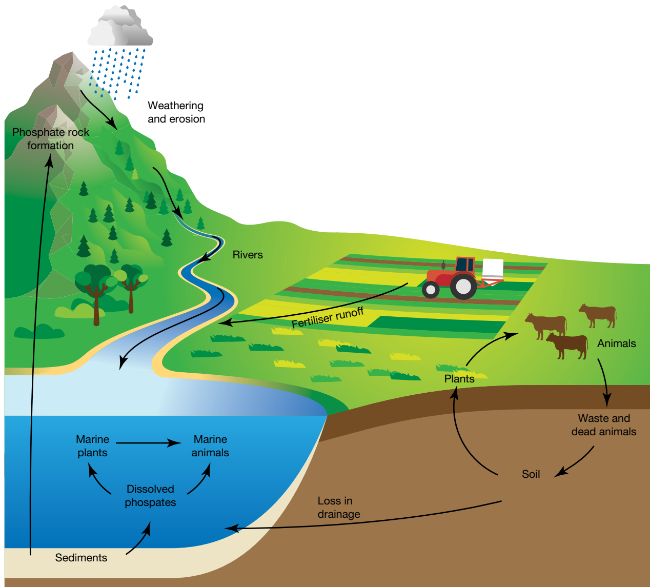
FIGURE 7.11 The phosphorus cycle
