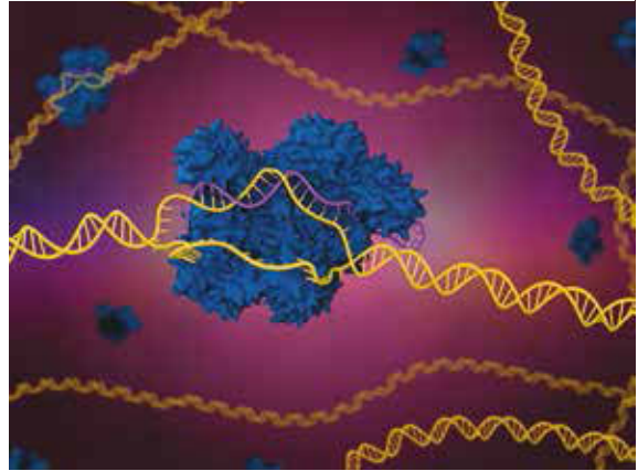
FIGURE 1.121 A target sequence (in purple) allows for the DNA to be cut at a specific location.
