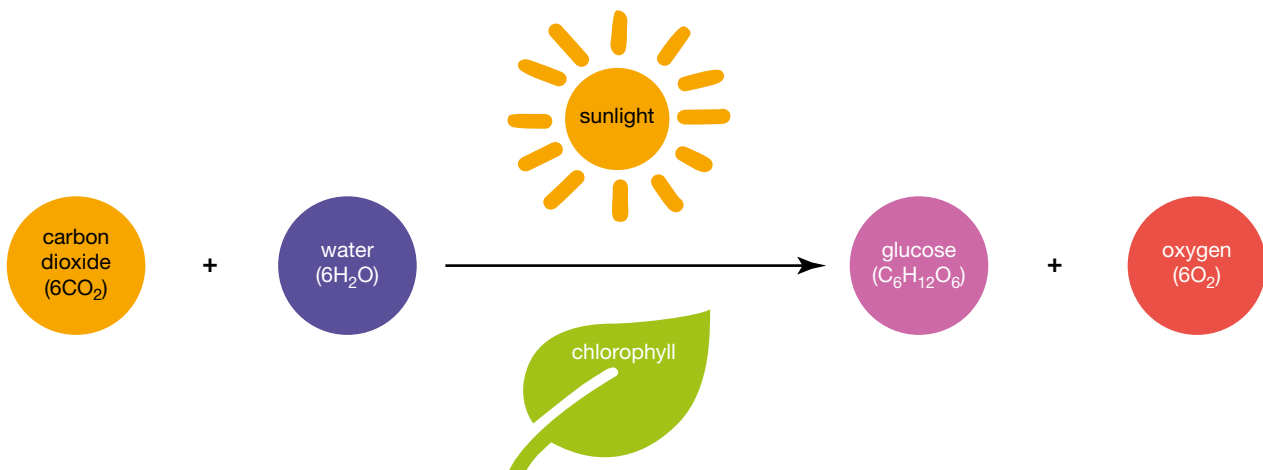
FIGURE 7.27 The process of photosynthesis
