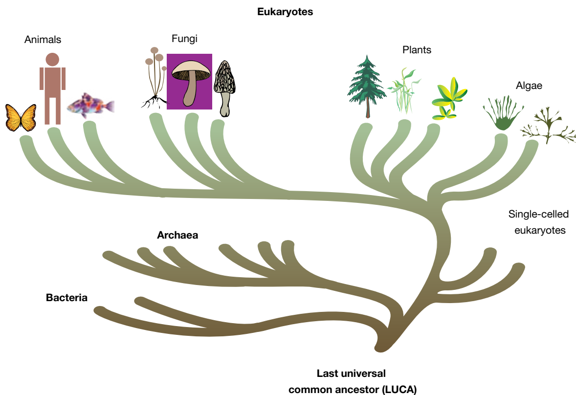
FIGURE 3.2 The theory of the last universal common ancestor
