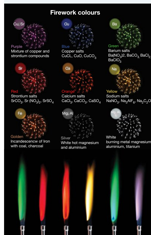
FIGURE 4.20 Fireworks use the principles of the flame test to produce many colours.
