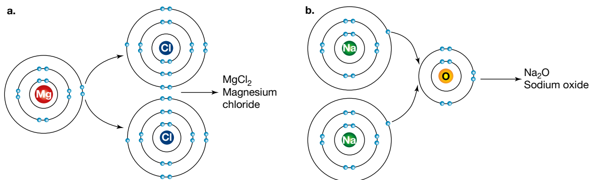
FIGURE 4.26 Electron transfer diagram involving more than two atoms. a. Magnesium chloride involves the two chlorine atoms each receiving an electron from magnesium, to form stable chloride ions. b. Sodium oxide involves two sodium atoms each giving their electron to oxygen, allowing it to form the stable oxide ion.
