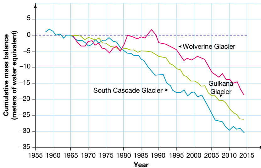
FIGURE 7.54 The change in mass of glaciers found in the US show a disturbing decrease in their size.
