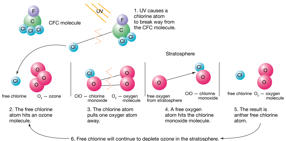
FIGURE 7.13 How CFCs break down and destroy ozone molecules
