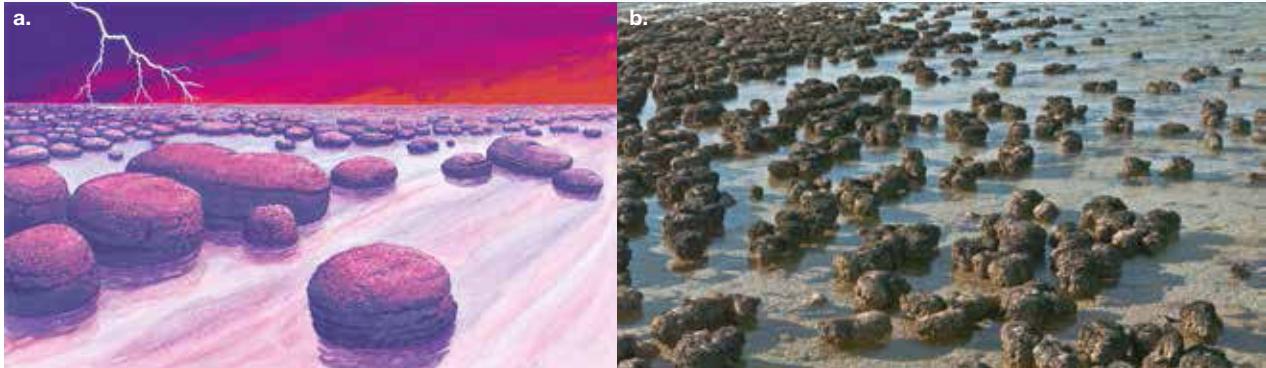
FIGURE 7.47 a. Earth was a hostile place 3500 million years ago. Fossils provide evidence of structures called stromatolites. They existed in warm sea water and consisted of cyanobacteria, one of the earliest forms of life. b. Stromatolites seen today in Shark Bay, Western Australia
