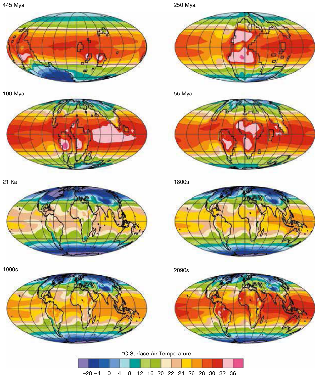
FIGURE 7.40 The study of paleoclimates throughout history may help us develop climate models to predict climates of the future. (Kya = thousand years ago; Mya = million years ago)
