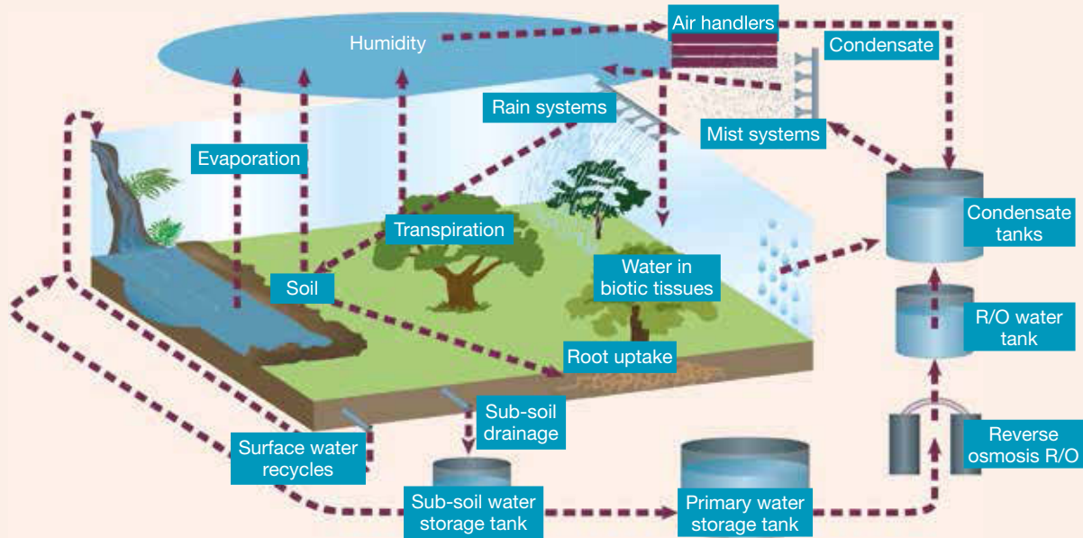
FIGURE 7.67 Water was conserved inside the Biosphere 2 wilderness environments. Condensation, artificial rain or irrigation (by sprinkler systems), evaporation, transpiration and sub-soil drainage were the major internal water cycling components.
