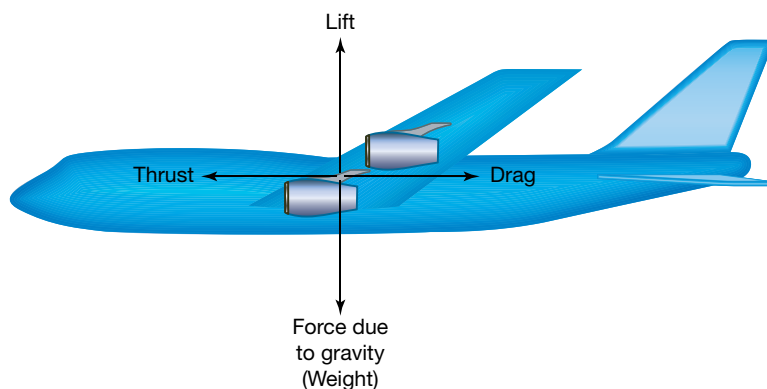
FIGURE 8.20 The plane flies at a steady speed because no unbalanced net force is acting on it.
