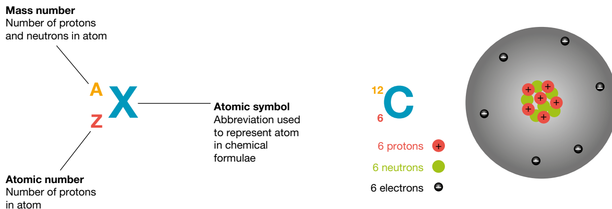
FIGURE 4.5 Notation used for atoms of different elements
