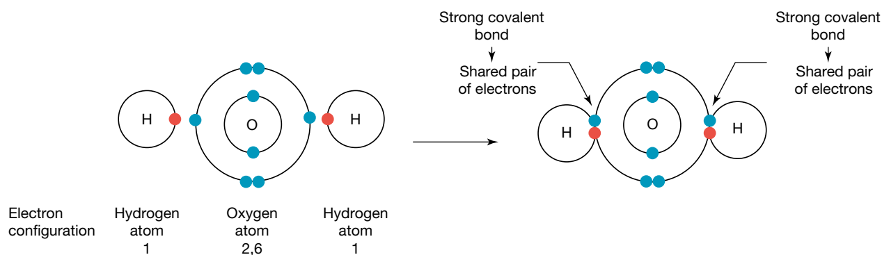
FIGURE 4.29 Formation of covalent bonds between hydrogen and oxygen atoms in a water molecule
