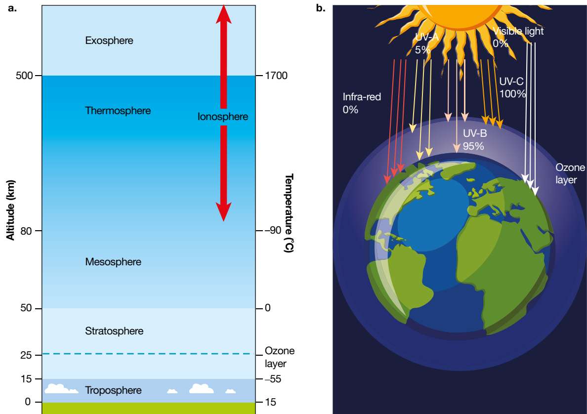
FIGURE 7.4 a. Layers in the Earth's atmosphere b. How the ozone layer in the stratosphere protects the Earth. The percentages show the amount of each type of radiation that is absorbed by the ozone layer.
