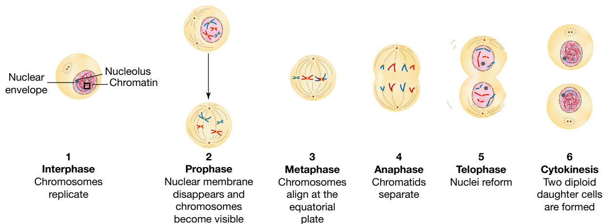
FIGURE 2.63 The stages of the cell cycle, including interphase, when DNA is replicated, and mitosis, when the nucleus divides
