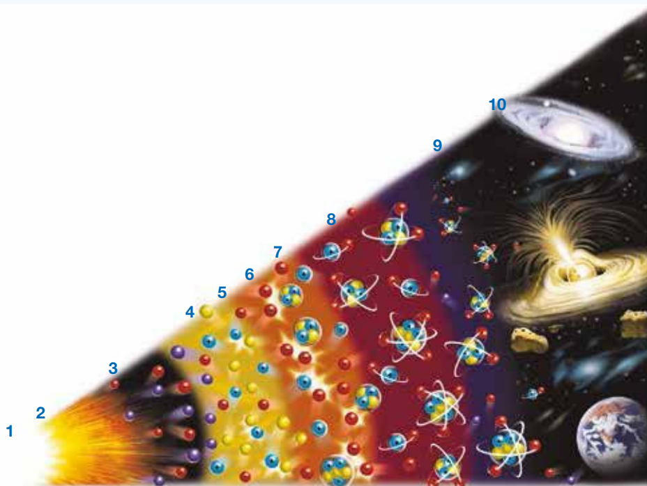
FIGURE 6.15 From the 'big bang' to one billion years old: the universe's formation according to the Big Bang theory
