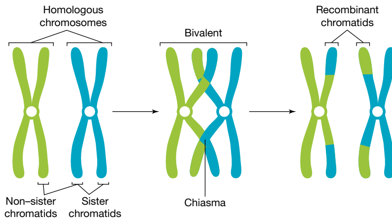
FIGURE 3.15 The process of crossing over
