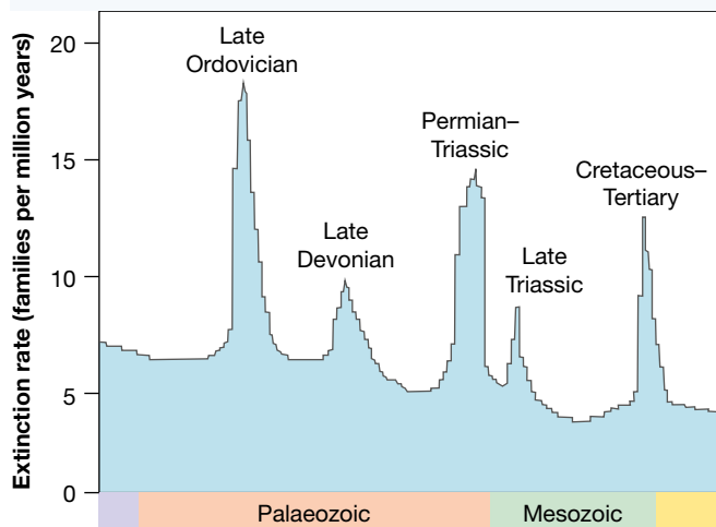
FIGURE 7.50 Five mass extinctions in the past
