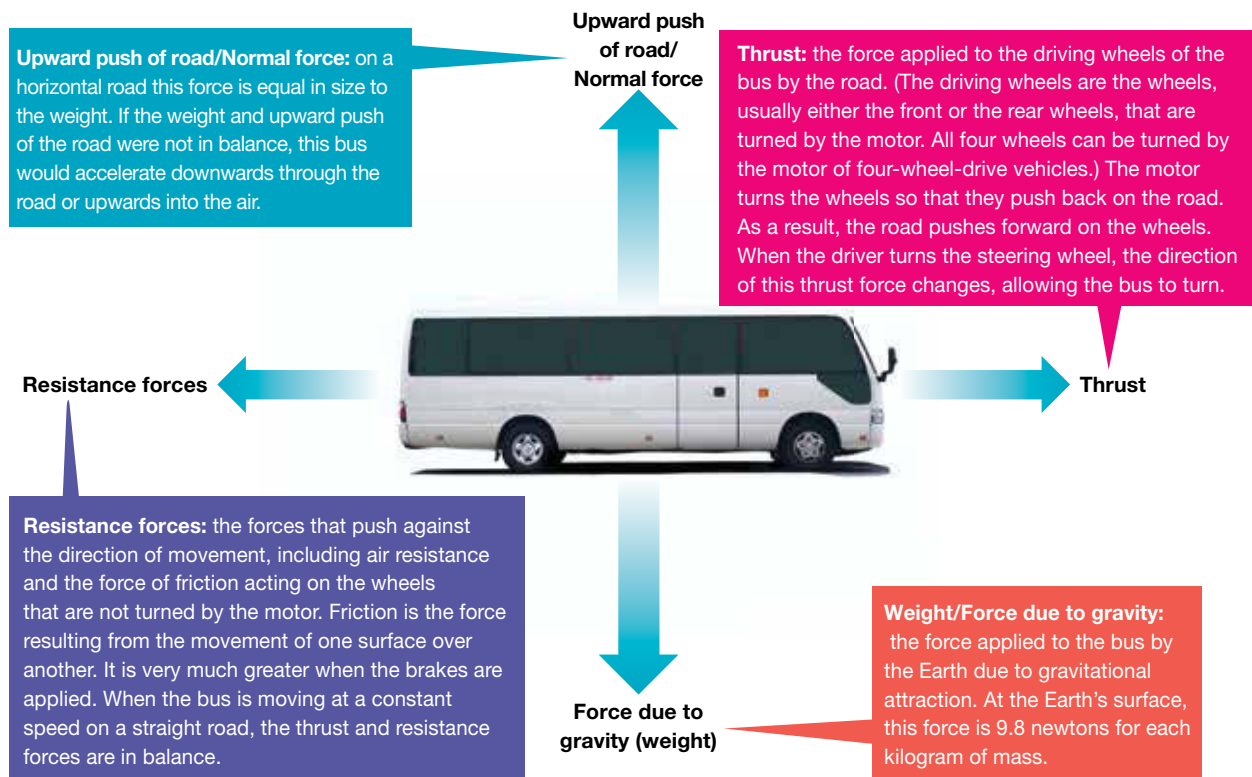
FIGURE 8.21 The forces acting on a moving bus. The forces are in balance when the bus is not changing speed or direction.
