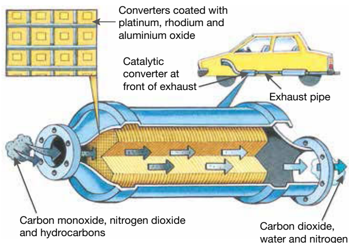
FIGURE 5.38 Catalytic converters have a large surface area and are coated with a metal catalyst.
