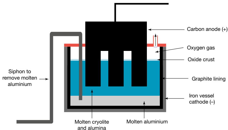
FIGURE 5.22 Extraction of aluminium using electrolysis
