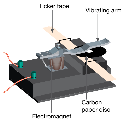
FIGURE 8.10 Motion can be recorded with a ticker timer.
