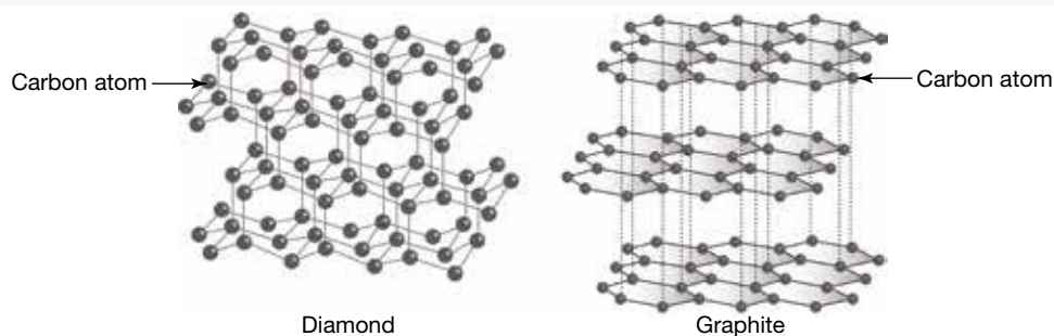
FIGURE 4.31 Different examples of covalent network lattices
