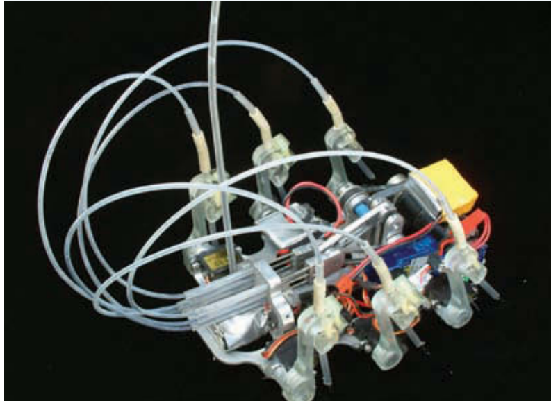
FIGURE 9.26 A model of the iSprawl
