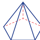
Pentagonal pyramid
