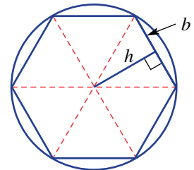
Hexagon ( n = 6 )
