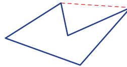
Non-convex polygon
