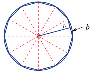
Dodecagon ( n = 12 )
