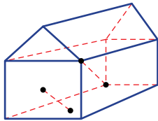
Convex solid
